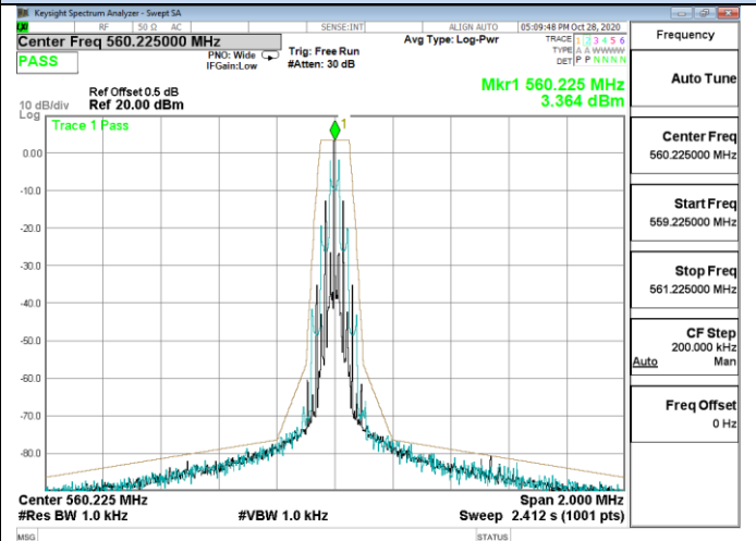
Channel 25 / 560.225 MHz
