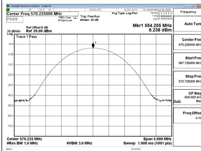
Channel 01 / 570.225 MHz
