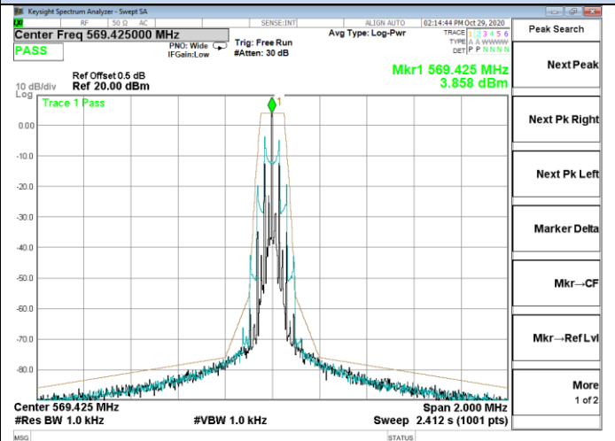
Channel 32 / 569.425 MHz
