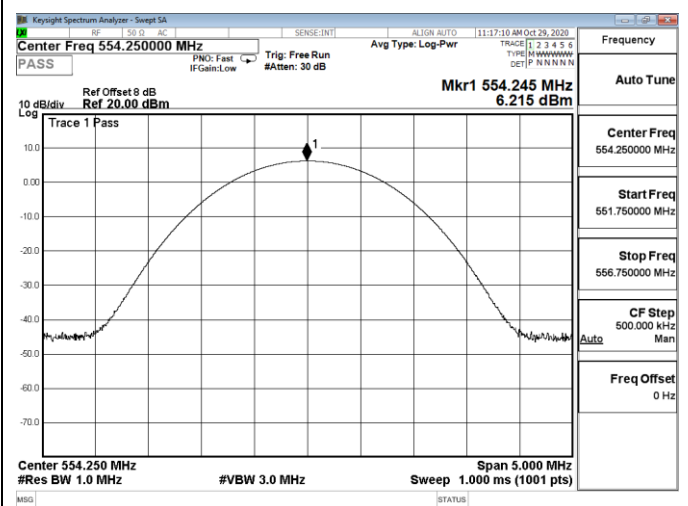
Channel 17 / 554.250 MHz
