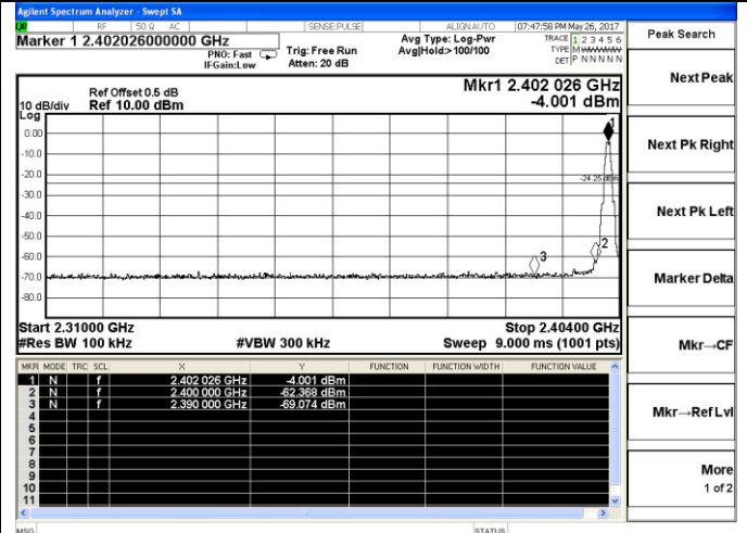
Channel 0 / 2402 MHz
