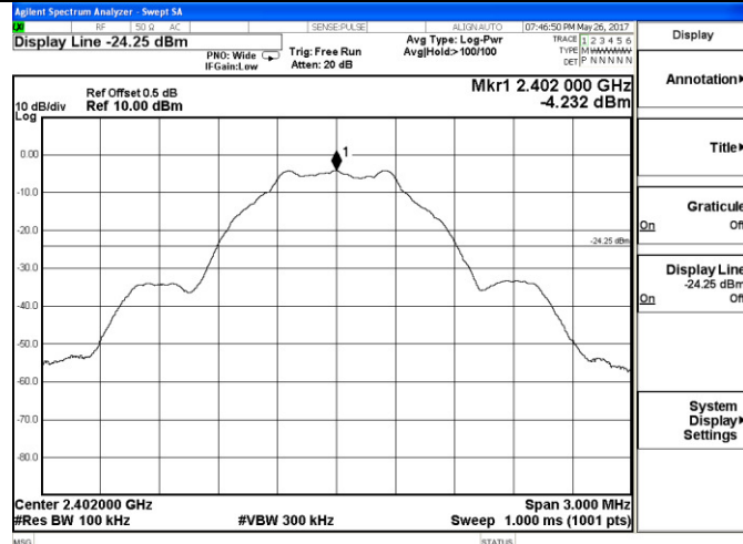
2401 – 2403 MHz
