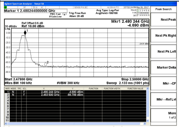
Channel 39 / 2480 MHz
