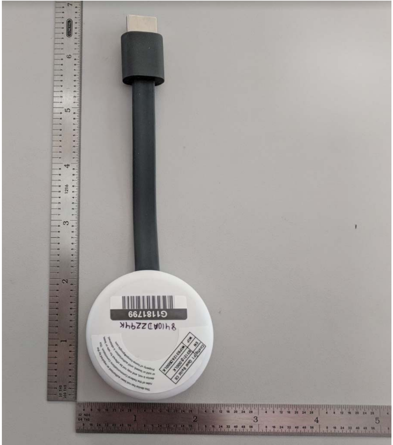
Bottom View
