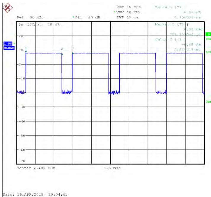
Time-domain plot for Bluetooth transmission signal
