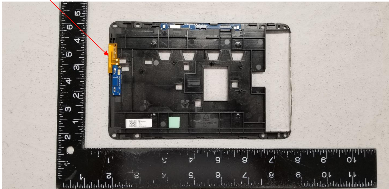
Antenna location
