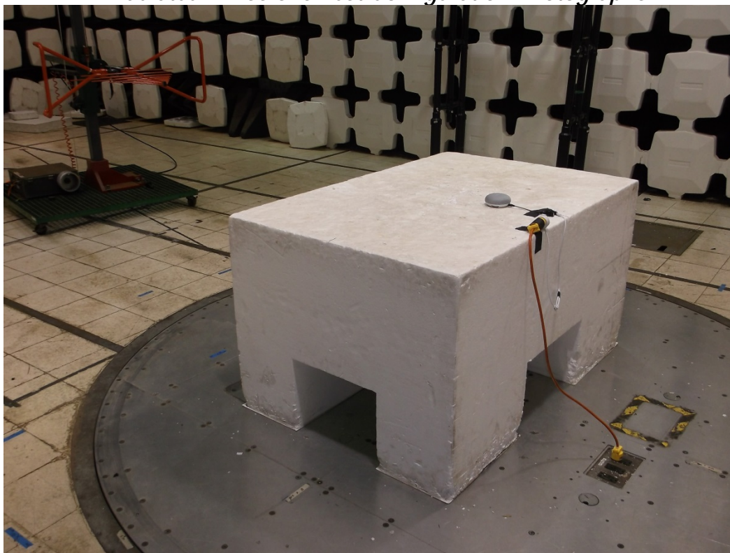
30 – 1000 MHz
