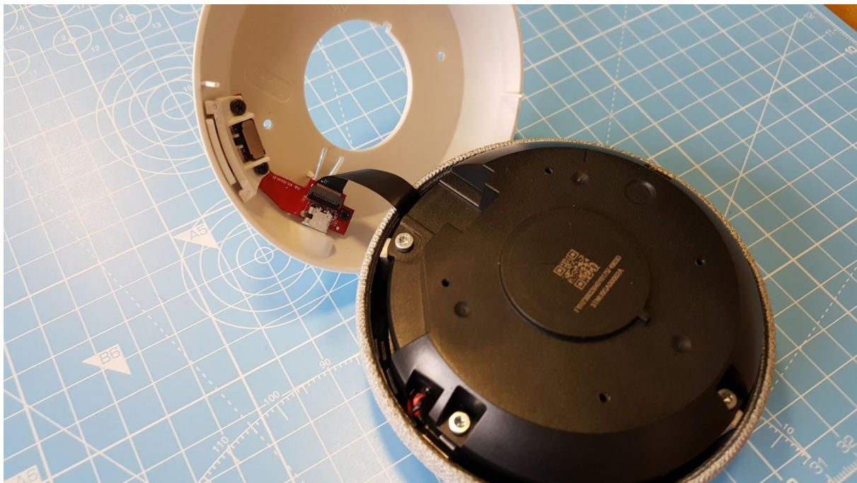
Speaker and Ribbon Cable to USB Port Close-up
