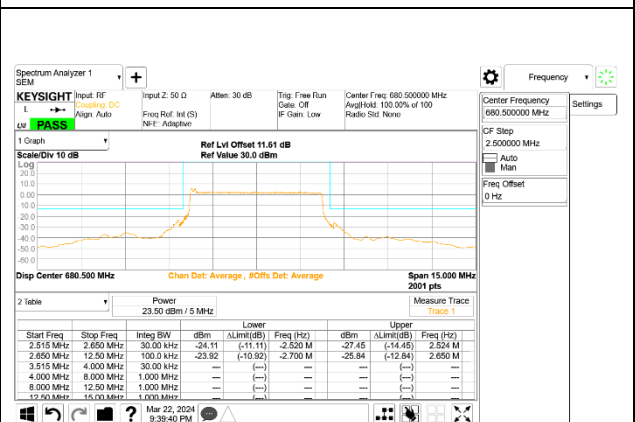
5G NR n71 5MHz BPSK Middle Channel RB25-0, ID:19210
