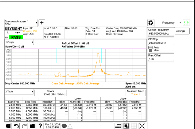
5G NR n71 5MHz BPSK Middle Channel RB1-24, ID:19210
