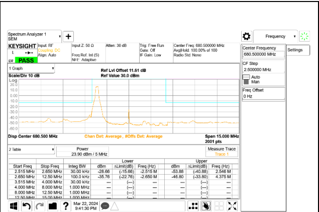
5G NR n71 5MHz BPSK Middle Channel RB1-0, ID:19210
