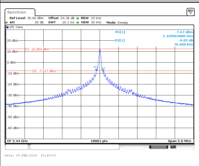
20 dB Bandwidth Plot in Channel 38
