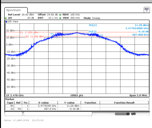
6 dB Bandwidth Plot on Channel 76
