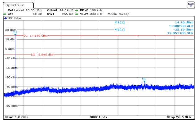
CSE Plot on High Ch between 1GHz ~ 26.5GHz
