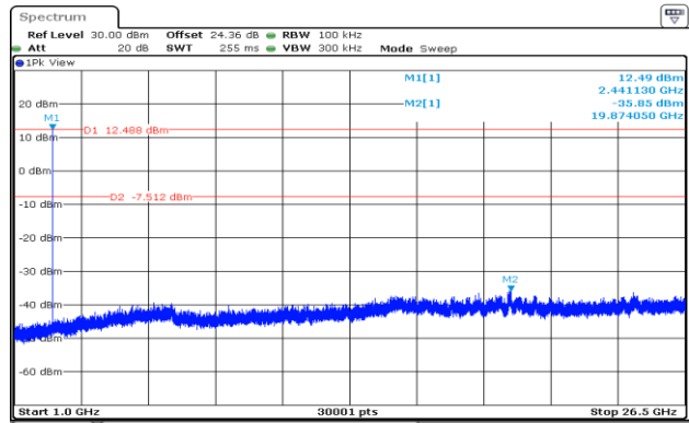
CSE Plot on Mid. Ch between 1GHz ~ 26.5GHz
