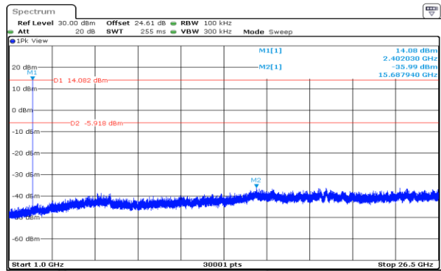
CSE Plot on Low Ch between 1GHz ~ 26.5GHz
