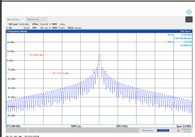
20 dB Bandwidth Plot in Channel 02
