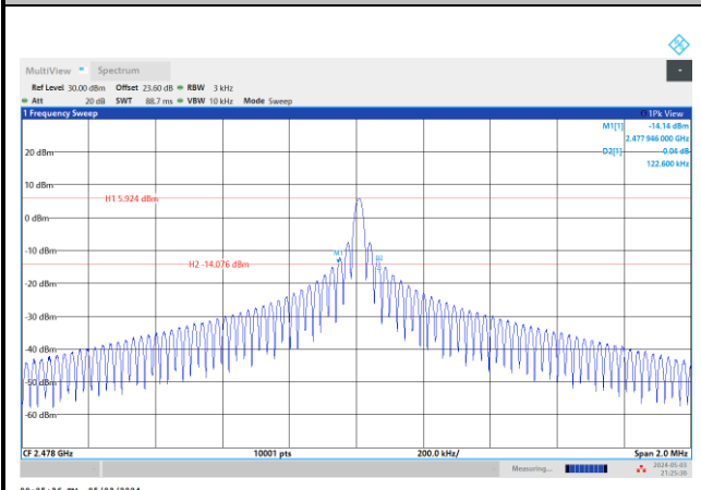
20 dB Bandwidth Plot in Channel 76
