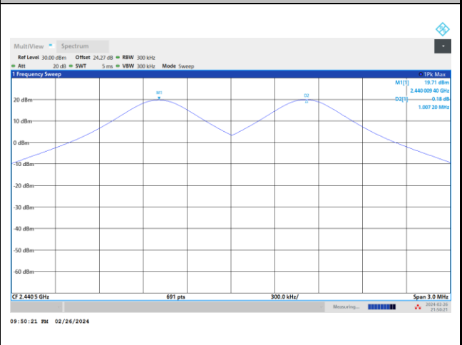
Channel Separation Plot on Channel 38 - 39
