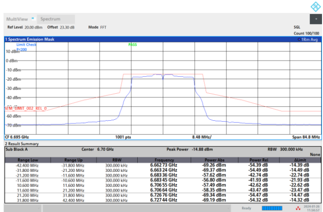
Plot on Channel 6695 MHz
