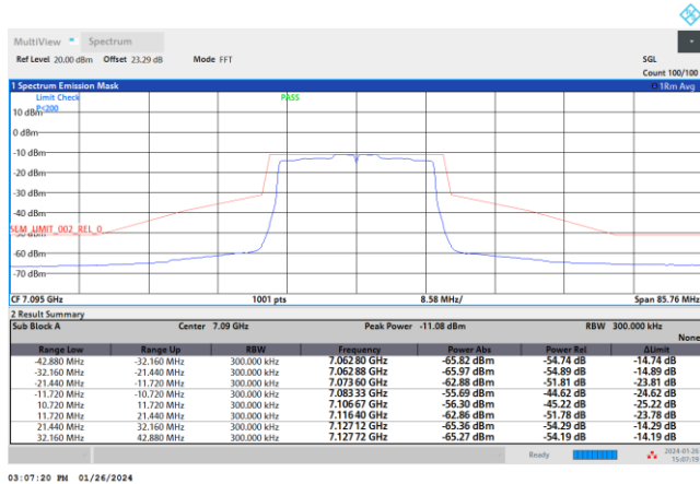
Plot on Channel 7095 MHz
