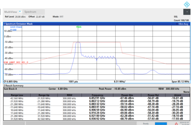
Plot on Channel 6895 MHz
