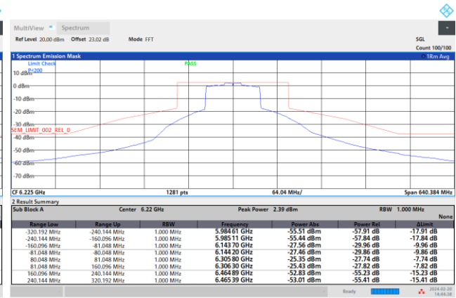
Plot on Channel 6225 MHz
