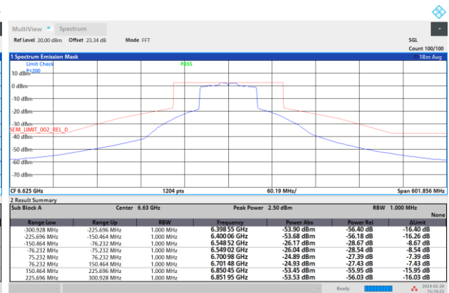
Plot on Channel 6625 MHz
