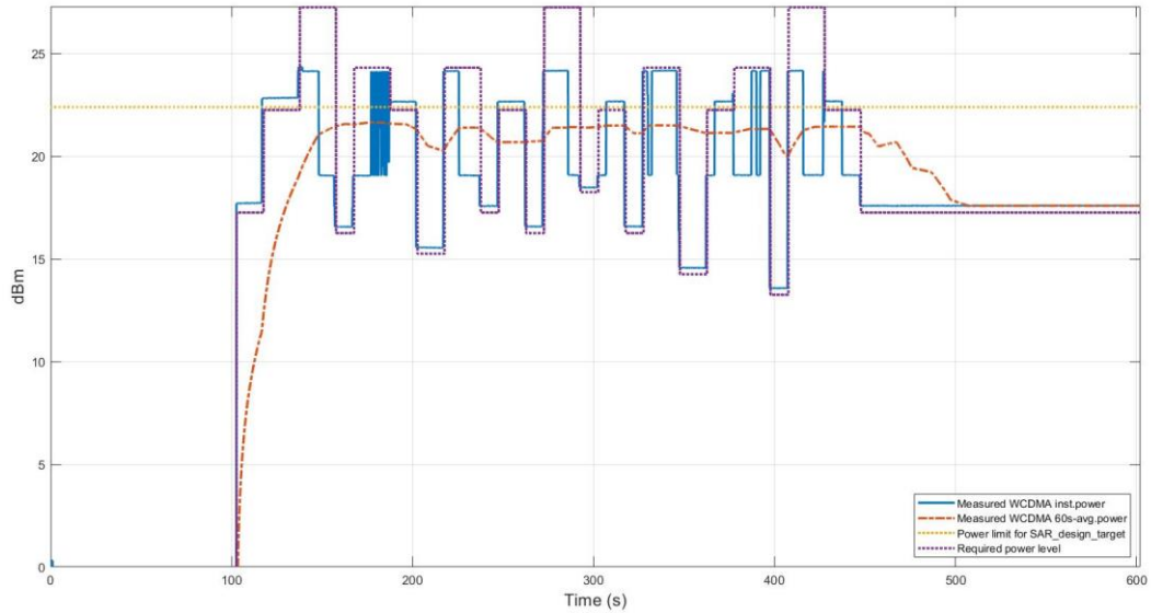
Figure 7.3-13 Conducted Tx power
