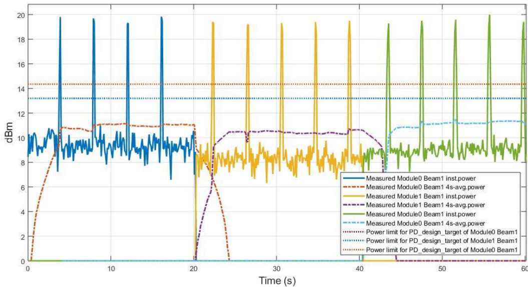
Figure 8.4-1 Measured radiated EIRP of FR2 n260 in mmWave Module beam change case F_TC03
