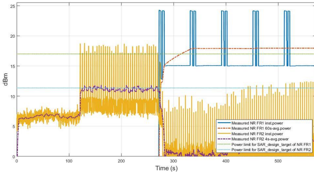
Figure 8.5-1 Measured radiated EIRP of FR2 n260 in mmWave Module beam change case TC04
