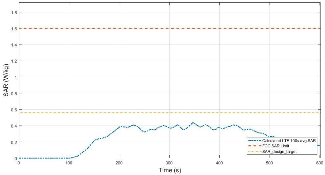
Figure 7.3-10 Total time-averaged SAR
