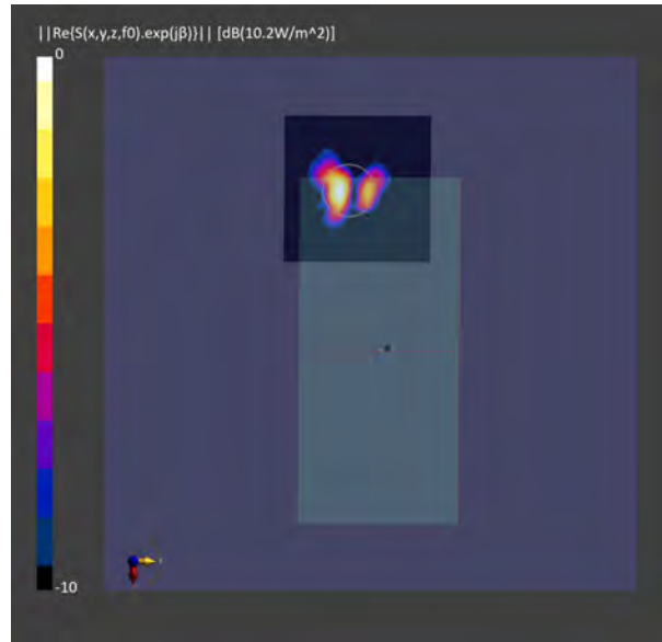
Figure 2-32 Simulated (left) and measured (right) PD distribution for the following configuration: Band n258, MID Channel, Beam ID 2, H polarization, Plane B Module, plotted on the surface S2 (back) with 2mm separation distance to the camera bump.
