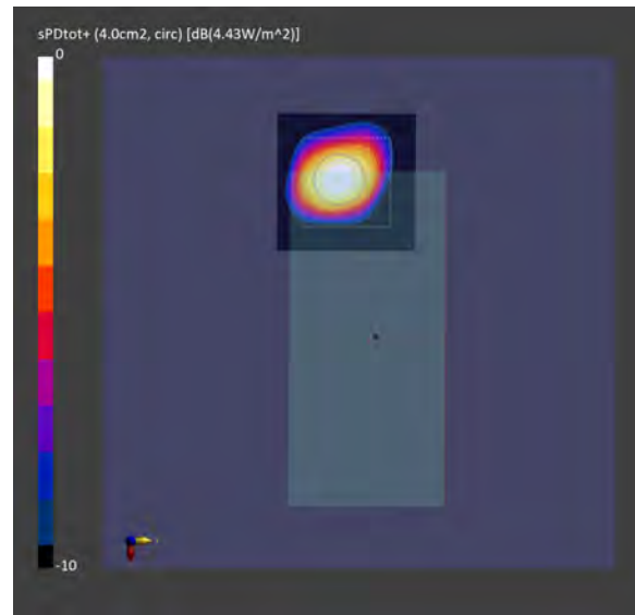
Figure 2-23 Simulated (left) and measured (right) averaged PD distribution for the following configuration: Band n261, MID Channel, Beam ID 4, V polarization, Plane B Module, plotted on the surface S2 (back) with 2mm separation distance to the camera bump.
