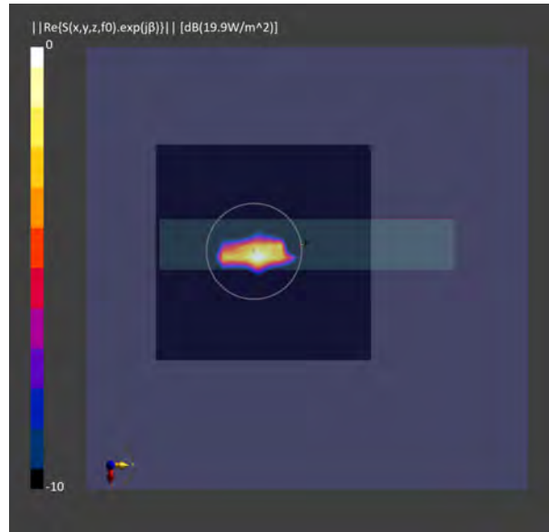
Figure 2-14 Simulated (left) and measured (right) PD distribution for the following configuration: Band n261, MID Channel, Beam ID 3, H polarization, Plane A Module, plotted on the surface S5 (top) with 2mm separation distance to the DUT.
