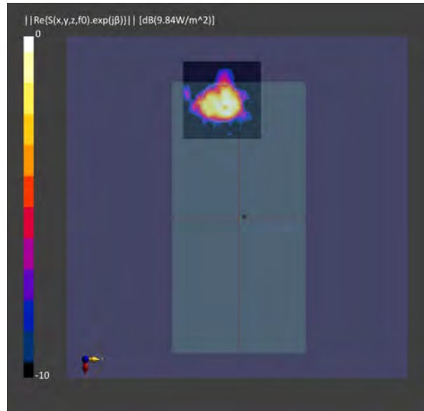
Figure 2-34 Simulated (left) and measured (right) PD distribution for the following configuration: Band n258, MID Channel, Beam ID 4, V polarization, Plane B Module, plotted on the surface S2 (back) with 2mm separation distance to the camera bump.
