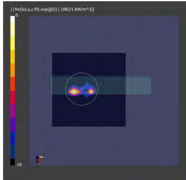
Figure 2-26 Simulated (left) and measured (right) PD distribution for the following configuration: Band n258, MID Channel, Beam ID 4, H polarization, Plane A Module, plotted on the surface S5 (top) with 2mm separation distance to the DUT.
