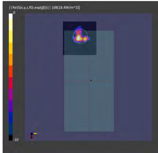
Figure 2-10 Simulated (left) and measured (right) PD distribution for the following configuration: Band n260, MID Channel, Beam ID 3, V polarization, Plane B Module, plotted on the surface S2 (back) with 2mm separation distance to the camera bump.
