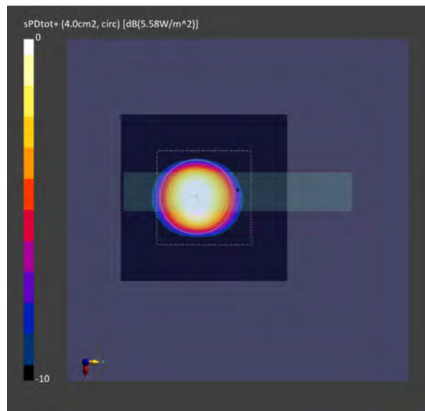
Figure 2-15 Simulated (left) and measured (right) averaged PD distribution for the following configuration: Band n261, MID Channel, Beam ID 3, H polarization, Plane A Module, plotted on the surface S5 (top) with 2mm separation distance to the DUT.
