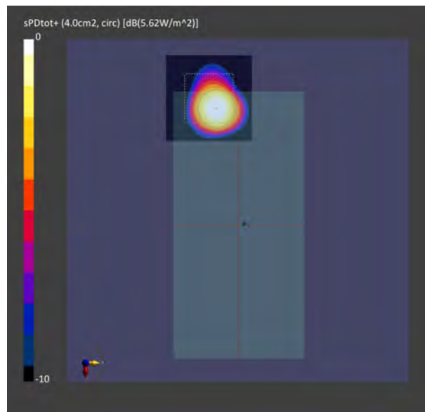
Figure 2-21 Simulated (left) and measured (right) averaged PD distribution for the following configuration: Band n261, MID Channel, Beam ID 2, H polarization, Plane B Module, plotted on the surface S2 (back) with 2mm separation distance to the camera bump.
