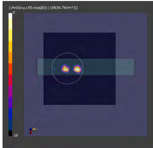
Figure 2-4 Simulated (left) and measured (right) PD distribution for the following configuration: Band n260, MID Channel, Beam ID 6, V polarization, Plane A Module, plotted on the surface S5 (top) with 2mm separation distance to the DUT.
