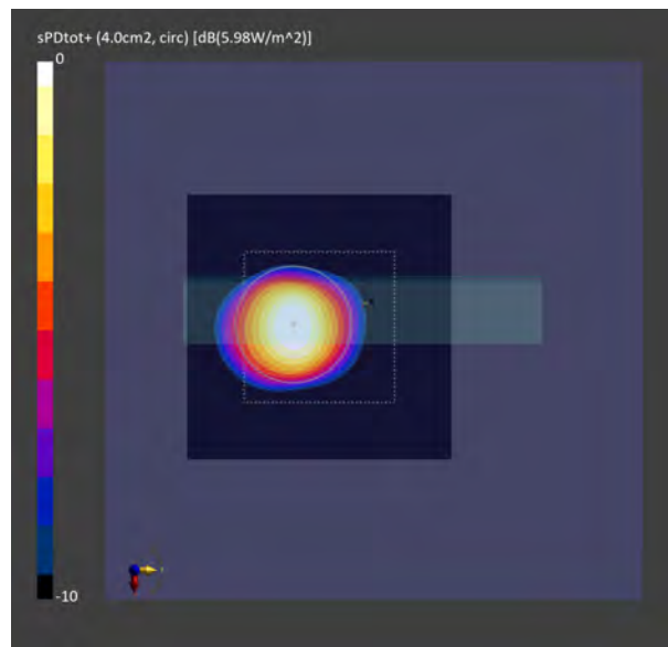
Figure 2-27 Simulated (left) and measured (right) averaged PD distribution for the following configuration: Band n258, MID Channel, Beam ID 4, H polarization, Plane A Module, plotted on the surface S5 (top) with 2mm separation distance to the DUT.
