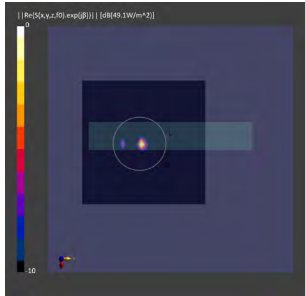
Figure 2-2 Simulated (left) and measured (right) PD distribution for the following configuration: Band n260, MID Channel, Beam ID 0, H polarization, Plane A Module, plotted on the surface S5 (top) with 2mm separation distance to the DUT.
