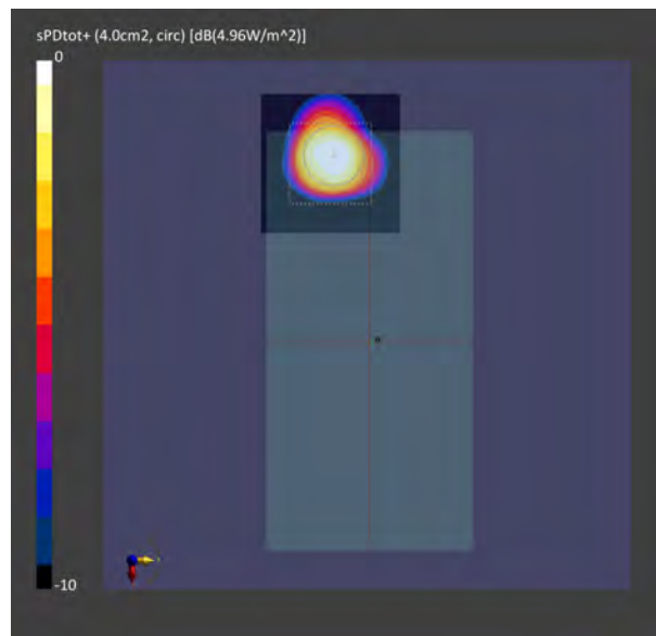
Figure 2-11 Simulated (left) and measured (right) averaged PD distribution for the following configuration: Band n260, MID Channel, Beam ID 3, V polarization, Plane B Module, plotted on the surface S2 (back) with 2mm separation distance to the camera bump.
