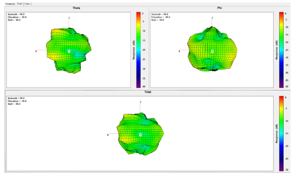
Ant3 Freq. 5180 MHz:
