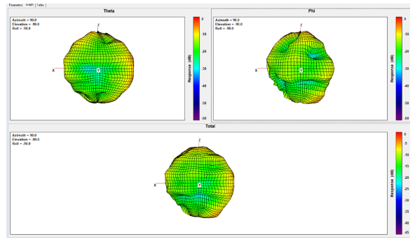
Ant4 Freq. 5500 MHz:
