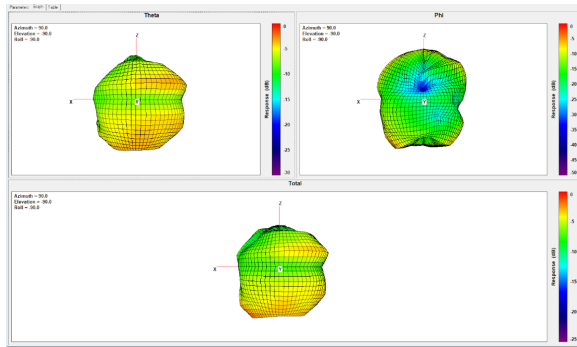
Ant3 Freq. 2437 MHz:
