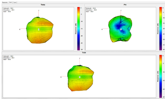
Ant3 Freq. 2462 MHz:
