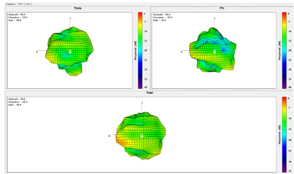
Ant3 Freq. 5500 MHz:
