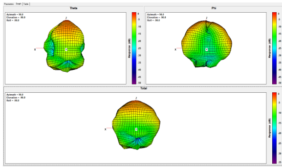
Ant4 Freq. 2462 MHz:
