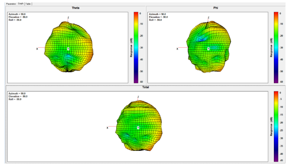
Ant4 Freq. 5887 MHz:
