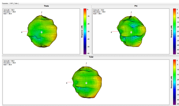
Ant4 Freq. 5280 MHz:
