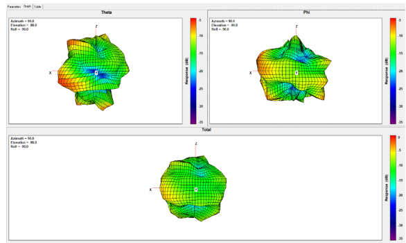
Ant3 Freq. 5280 MHz:
