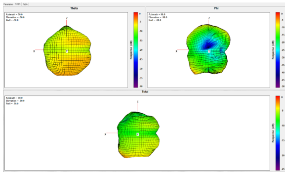
Ant3 Freq. 2412 MHz:
