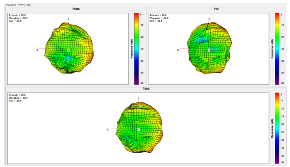
Ant4 Freq. 5820 MHz:
