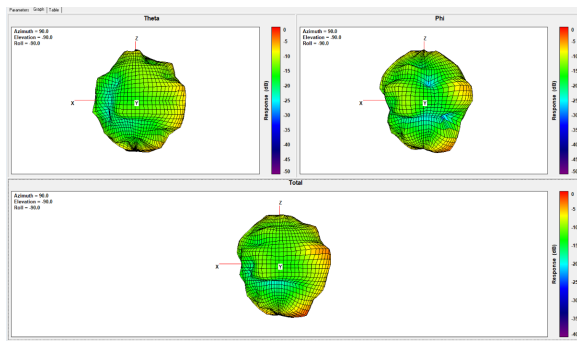
Ant4 Freq. 5180 MHz:
