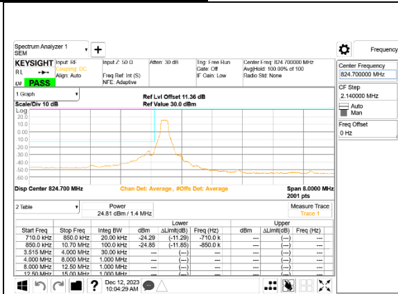
LTE B5 1.4MHz QPSK Low Channel RB1-0, ID:32061
