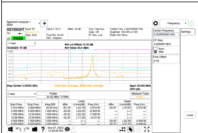
LTE B7 5MHz QPSK Low Channel RB1-24, ID:39005
