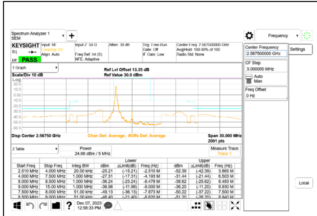
LTE B7 5MHz QPSK High Channel RB1-0, ID:39005
