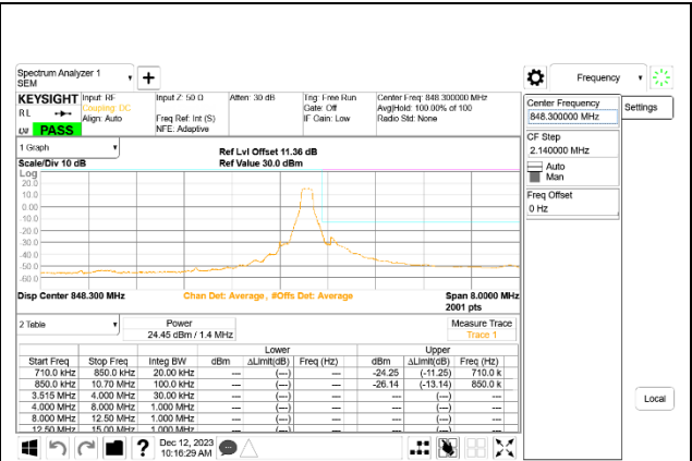
LTE B5 1.4MHz QPSK High Channel RB1-5, ID:32061
