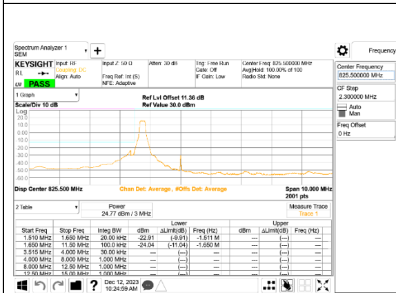
LTE B5 3MHz QPSK Low Channel RB1-0, ID:32061
