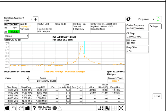
LTE B5 3MHz QPSK High Channel RB1-14, ID:32061
