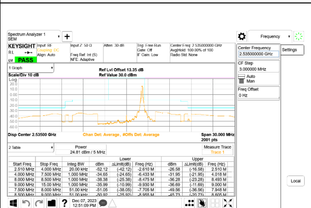
LTE B7 5MHz QPSK Middle Channel RB1-24, ID:39005
