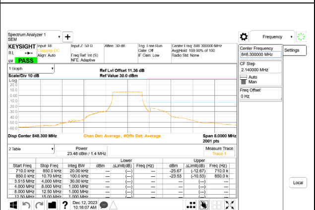
LTE B5 1.4MHz QPSK High Channel RB6-0, ID:32061
