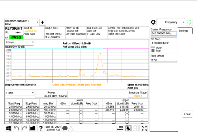
5G NR n5 5MHz BPSK High Channel RB1-24, ID:24898
