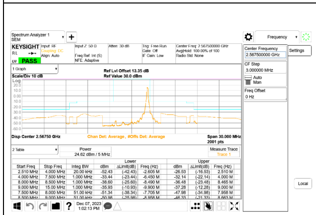
LTE B7 5MHz QPSK High Channel RB1-24, ID:39005
