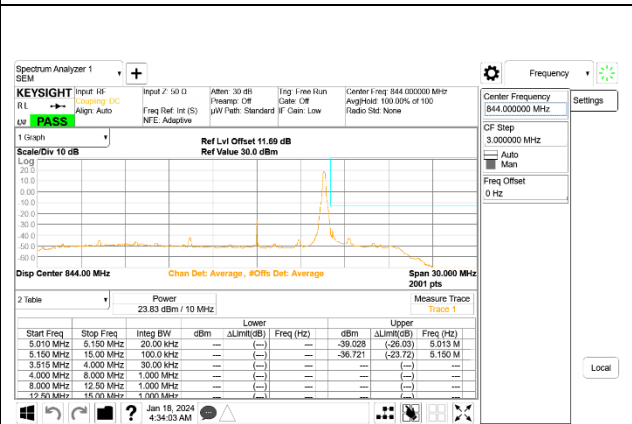
5G NR n5 10MHz BPSK High Channel RB1-51, ID:24898
