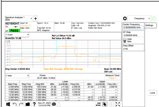
LTE B7 5MHz QPSK Low Channel RB25-0, ID:39005
