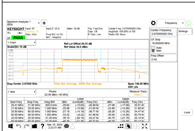
5G NR n41 40MHz BPSK High Channel RB100-0, ID:24898
