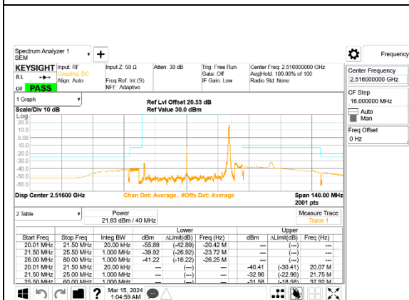
5G NR n41 40MHz BPSK Low Channel RB1-105, ID:24898
