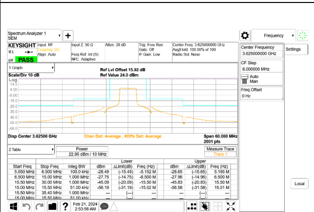
LTE B48 5MHz QPSK Middle Channel RB25-0, ID:19210
