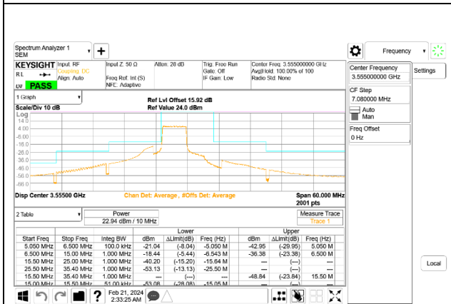
LTE B48 5MHz QPSK Low Channel RB25-0, ID:19210
