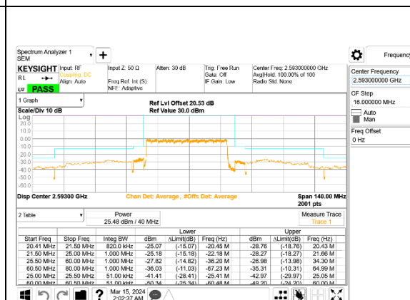
5G NR n41 40MHz BPSK Middle Channel RB100-0, ID:24898
