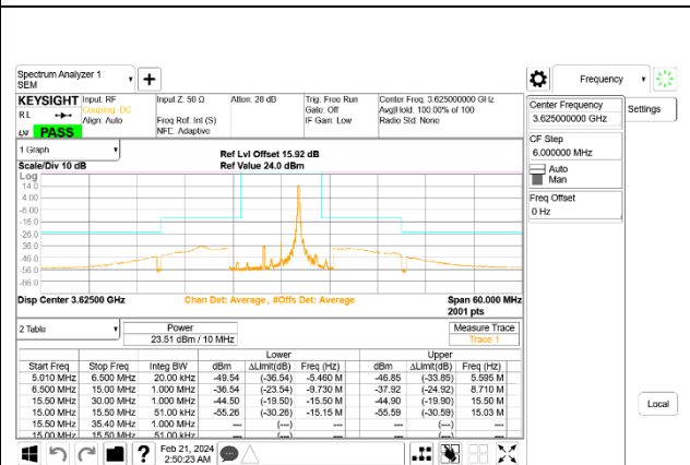
LTE B48 5MHz QPSK Middle Channel RB1-24, ID:19210
