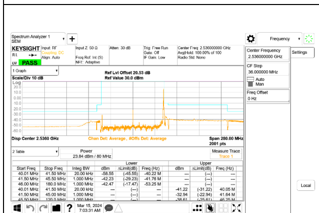
5G NR n41 80MHz BPSK Low Channel RB1-216, ID:24898
