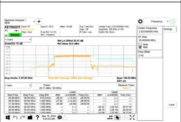
5G NR n41 50MHz BPSK Low Channel RB128-0, ID:24898
