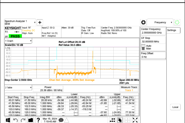
5G NR n41 80MHz BPSK Middle Channel RB1-216, ID:24898
