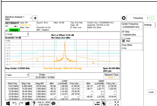
LTE B48 5MHz QPSK Low Channel RB1-24, ID:19210
