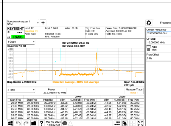
5G NR n41 40MHz BPSK Middle Channel RB1-105, ID:24898
