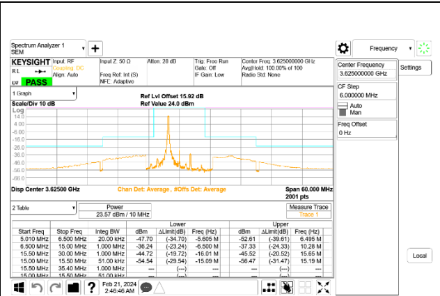
LTE B48 5MHz QPSK Middle Channel RB1-0, ID:19210
