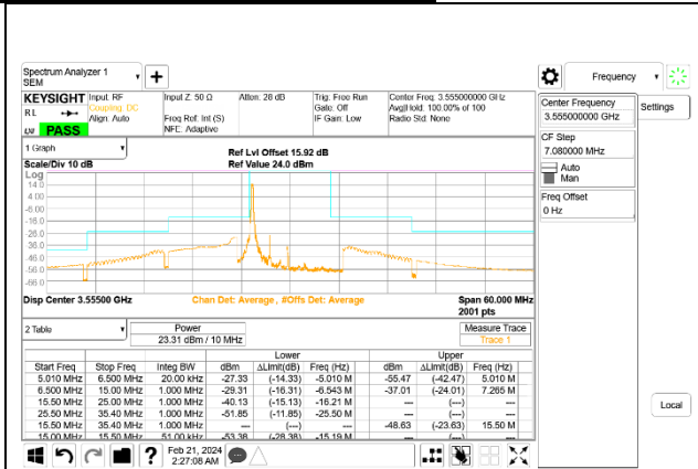
LTE B48 5MHz QPSK Low Channel RB1-0, ID:19210
