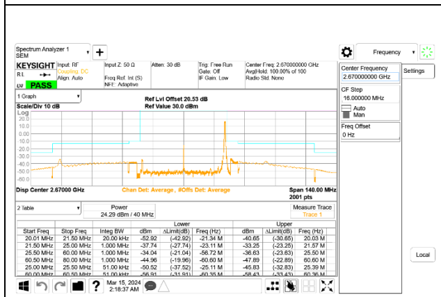
5G NR n41 40MHz BPSK High Channel RB1-105, ID:24898
