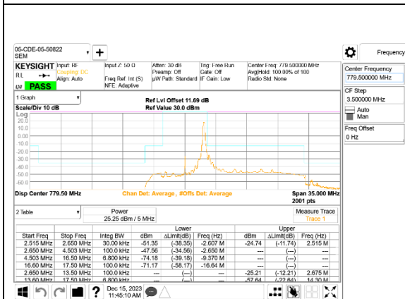
LTE B13 5MHz QPSK Low Channel RB1-24
