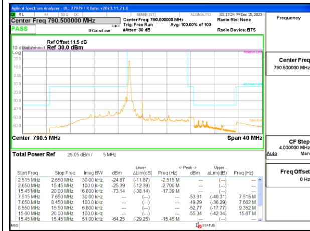
LTE B14 5MHz QPS Low Channel RB1-0, ID:27979
