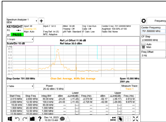
LTE B12 5MHz QPSK Low Channel RB1-0, ID:25780
