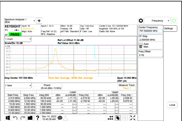
LTE B12 5MHz QPSK Middle Channel RB1-0, ID:25780
