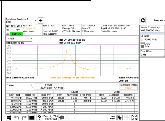
LTE B12 1.4MHz QPSK Low Channel RB1-0, ID:25780
