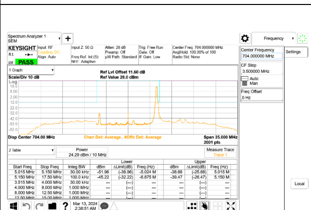
5G NR n12 10MHz BPSK Low Channel RB1-51, ID:28498
