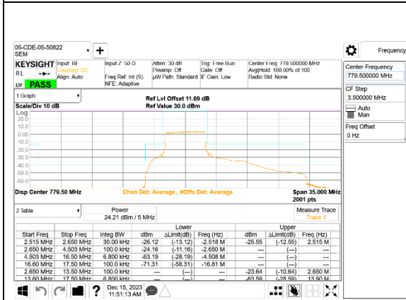
LTE B13 5MHz QPSK Low Channel RB25-0
