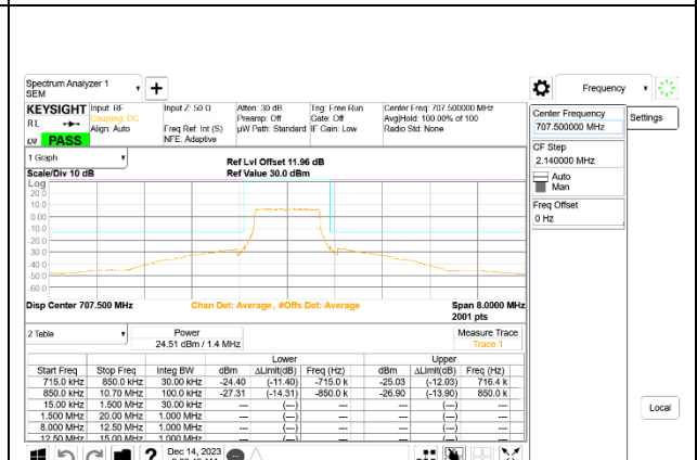
LTE B12 1.4MHz QPSK Middle Channel RB6-0, ID:25780
