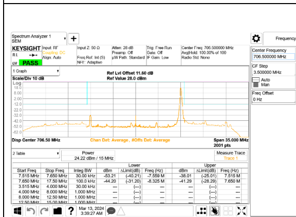
5G NR n12 15MHz BPSK Low Channel RB1-78, ID:28498
