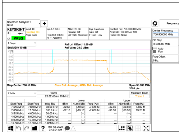
5G NR n12 15MHz BPSK Low Channel RB75-0, ID:28498
