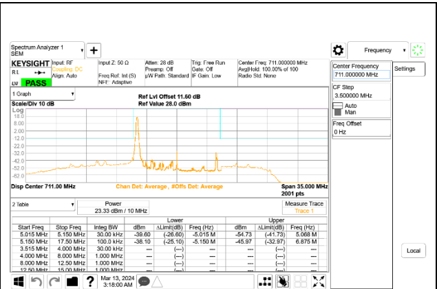
5G NR n12 10MHz BPSK High Channel RB1-0, ID:28498
