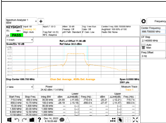
LTE B12 1.4MHz QPSK Low Channel RB6-0, ID:25780
