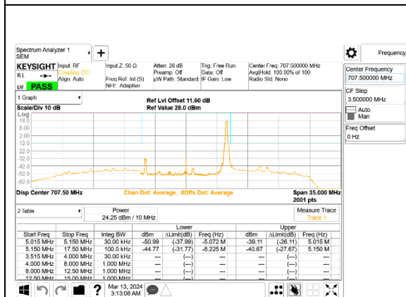
5G NR n12 10MHz BPSK Middle Channel RB1-51, ID:28498
