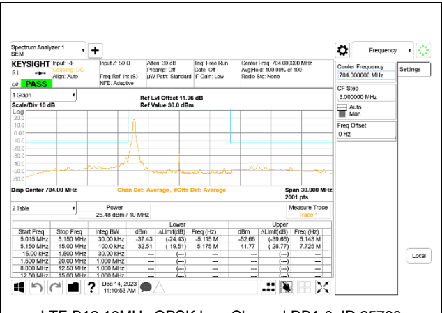
LTE B12 10MHz QPSK Low Channel RB1-0, ID:25780
