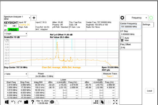
5G NR n12 5MHz BPSK Middle Channel RB1-0, ID:28498
