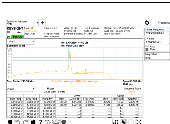
5G NR n12 5MHz BPSK High Channel RB1-0, ID:28498
