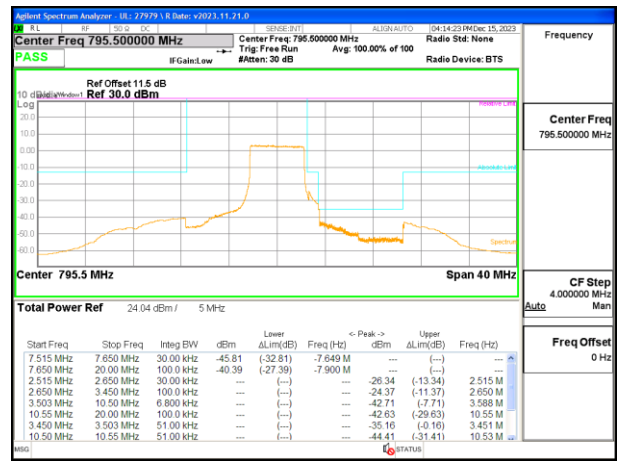
LTE B14 5MHz QPSK High Channel RB25-0, ID:27979
