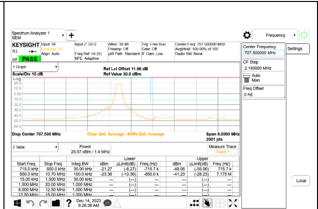
LTE B12 1.4MHz QPSK Middle Channel RB1-0, ID:25780
