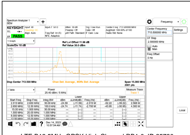
LTE B12 5MHz QPSK High Channel RB1-0, ID:25780
