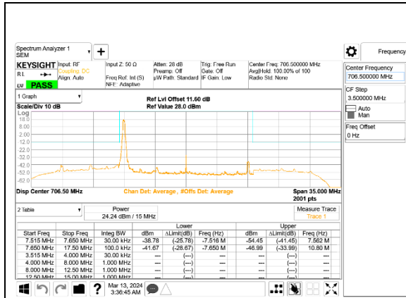
5G NR n12 15MHz BPSK Low Channel RB1-0, ID:28498
