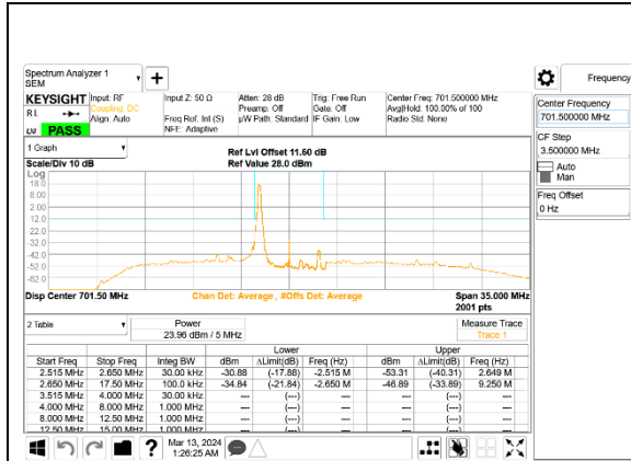
5G NR n12 5MHz BPSK Low Channel RB1-0, ID:28498
