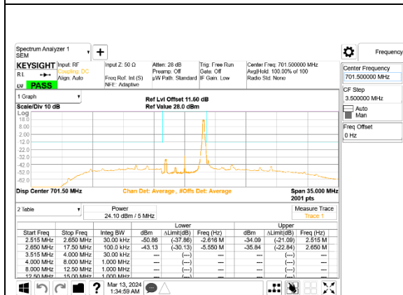
5G NR n12 5MHz BPSK Low Channel RB1-24, ID:28498
