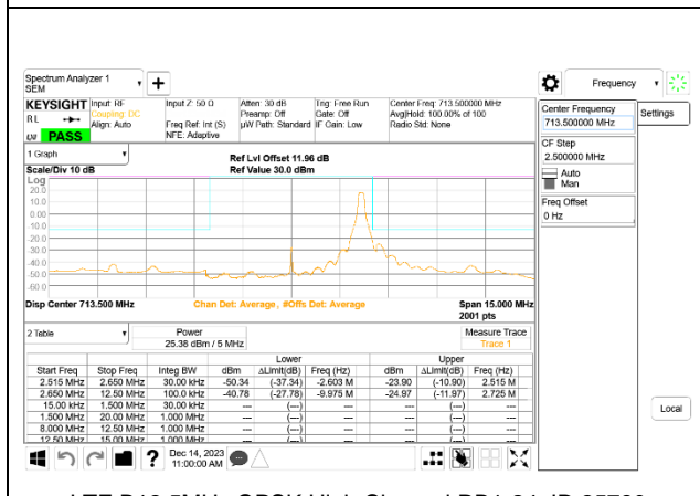
LTE B12 5MHz QPSK High Channel RB1-24, ID:25780
