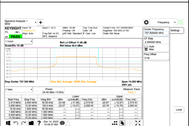
LTE B12 5MHz QPSK Middle Channel RB25-0, ID:25780
