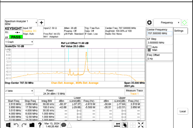
5G NR n12 5MHz BPSK Middle Channel RB1-24, ID:28498
