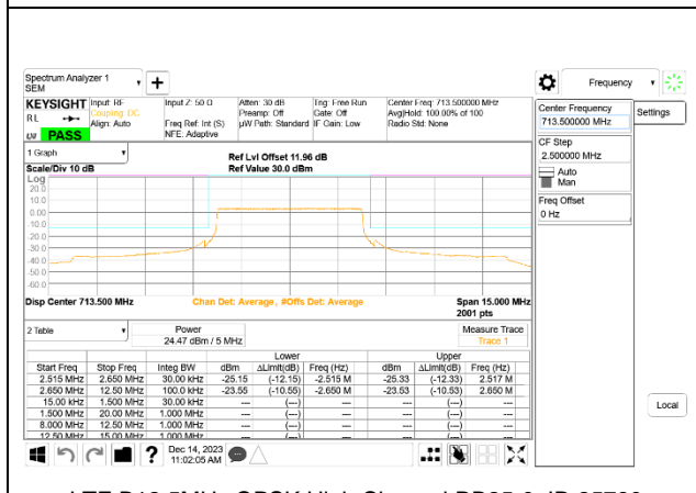
LTE B12 5MHz QPSK High Channel RB25-0, ID:25780
