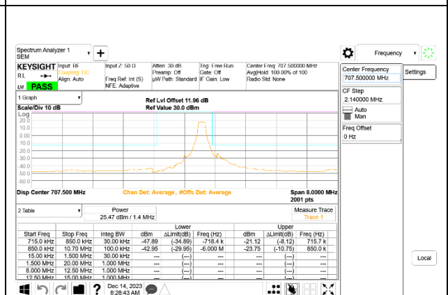
LTE B12 1.4MHz QPSK Middle Channel RB1-5, ID:25780
