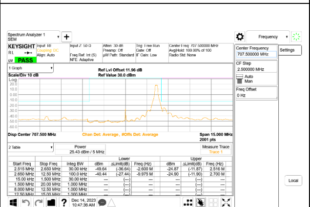
LTE B12 5MHz QPSK Middle Channel RB1-24, ID:25780
