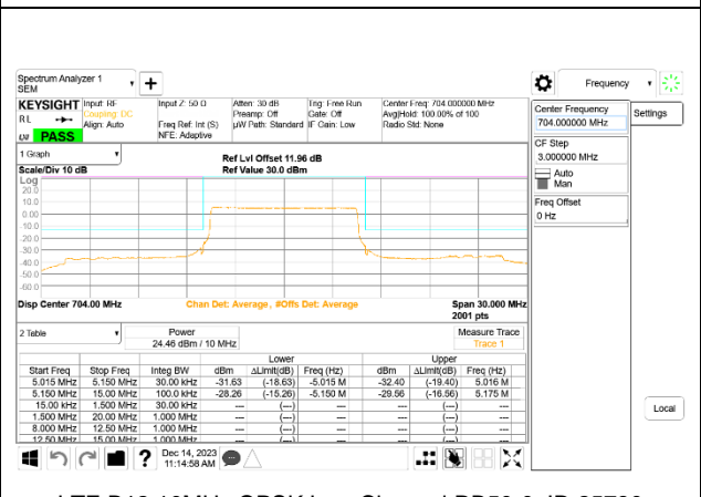
LTE B12 10MHz QPSK Low Channel RB50-0, ID:25780
