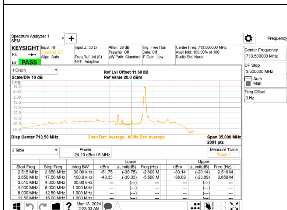
5G NR n12 5MHz BPSK High Channel RB1-24, ID:28498
