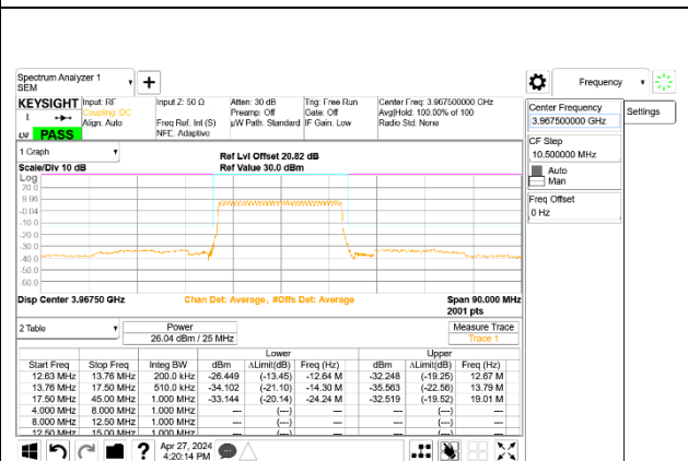
5G NR n77 25MHz BPSK High Channel RB64-0, ID:27966
