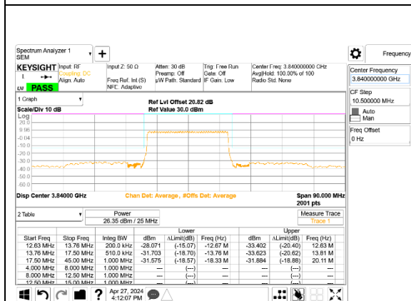
5G NR n77 25MHz BPSK Middle Channel RB64-0, ID:27966
