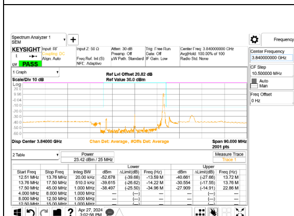
5G NR n77 25MHz BPSK Middle Channel RB1-64, ID:27966
