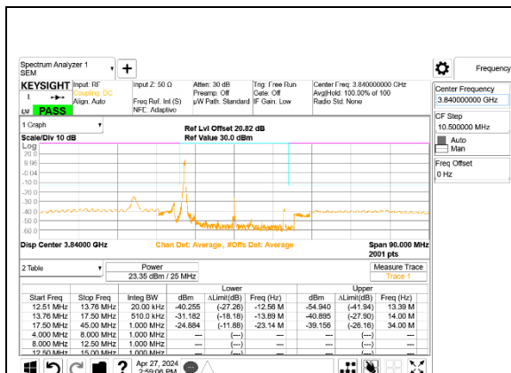
5G NR n77 25MHz BPSK Middle Channel RB1-0, ID:27966
