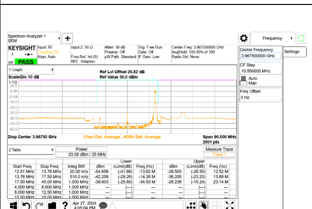
5G NR n77 25MHz BPSK High Channel RB1-64, ID:27966
