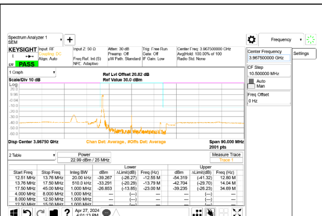
5G NR n77 25MHz BPSK High Channel RB1-0, ID:27966
