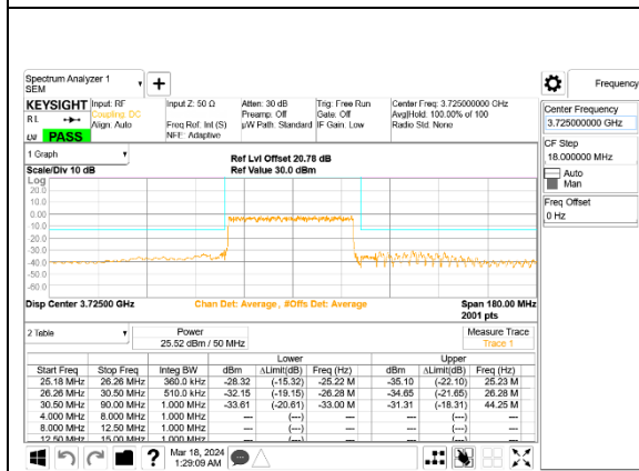
5G NR n77 50MHz BPSK Low Channel RB128-0, ID:28498
