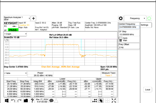
5G NR n77 40MHz BPSK Low Channel RB100-0, ID:28498
