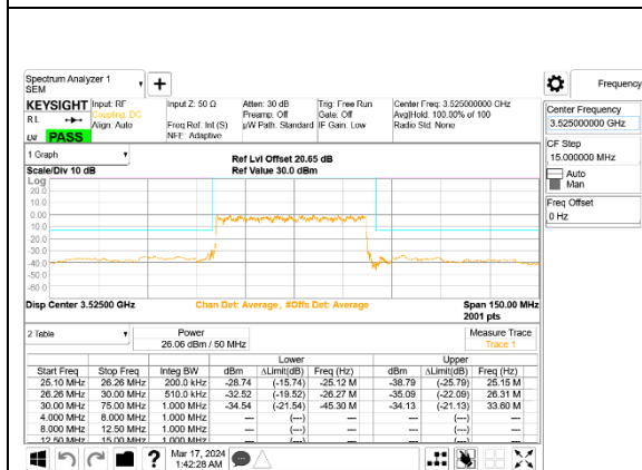
5G NR n77 50MHz BPSK High Channel RB128-0, ID:28498
