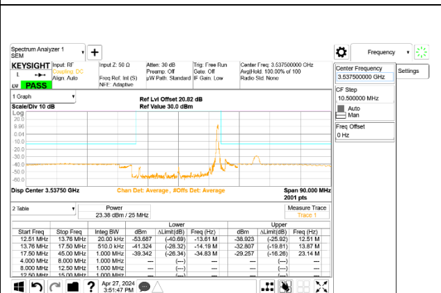
5G NR n77 25MHz BPSK High Channel RB1-64, ID:28498
