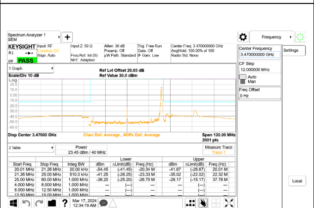
5G NR n77 40MHz BPSK Low Channel RB1-105, ID:28498
