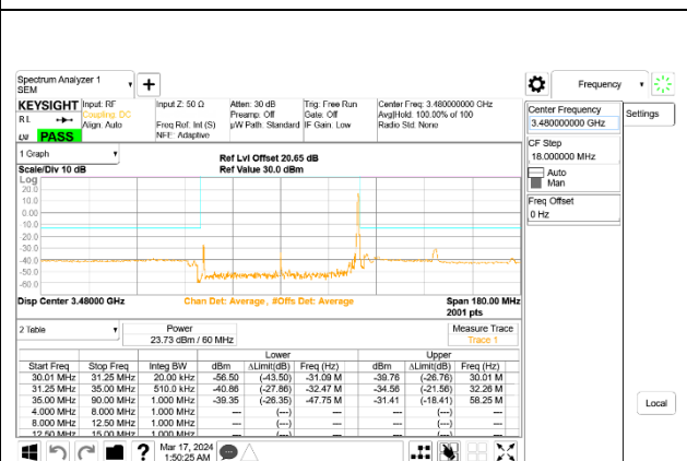
5G NR n77 60MHz BPSK Low Channel RB1-161, ID:28498
