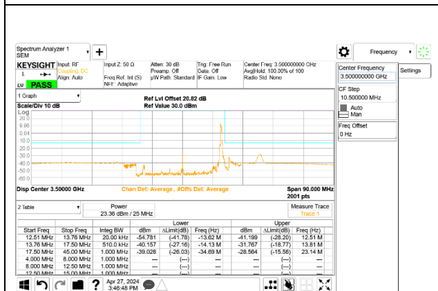
5G NR n77 25MHz BPSK Middle Channel RB1-64, ID:28498
