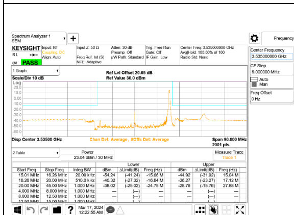
5G NR n77 30MHz BPSK High Channel RB1-77, ID:28498
