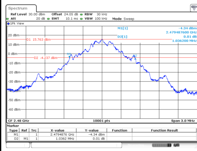
20 dB Bandwidth Plot in Channel 78
