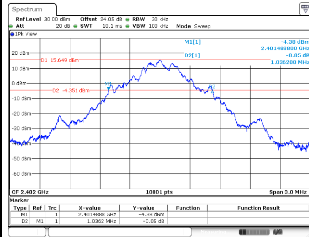
20 dB Bandwidth Plot in Channel 00
