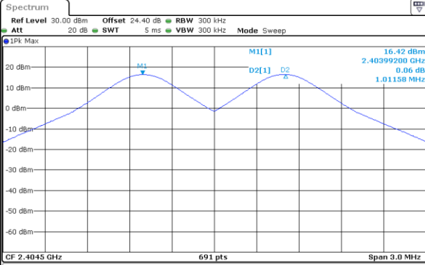
Channel Separation Plot on Channel 02 - 03
