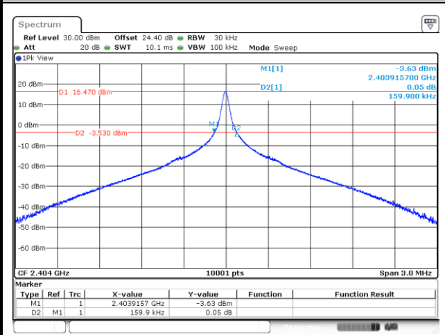
20 dB Bandwidth Plot in Channel 02
