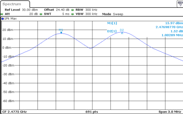
Channel Separation Plot on Channel 75 - 76
