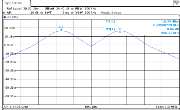
Channel Separation Plot on Channel 38 - 39
