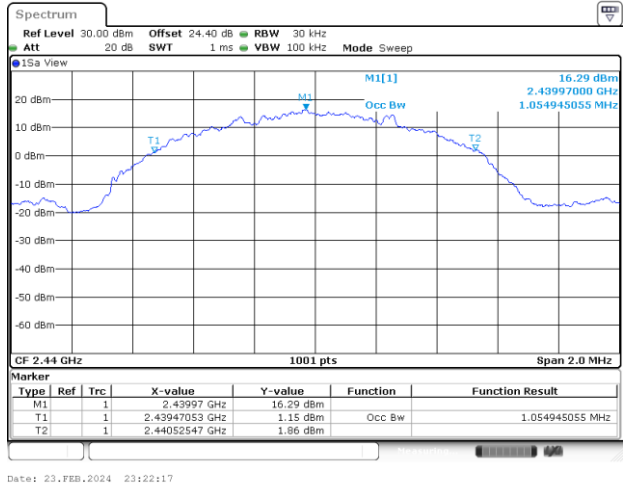
99% Occupied Plot Bandwidth on Channel 38
