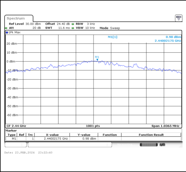
Power Density (dBm/3kHz) Plot Channel 38
