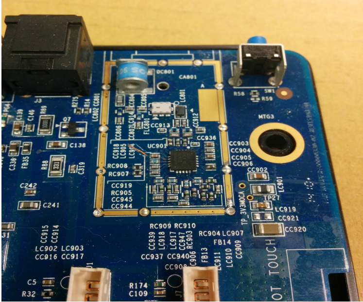
Top of PCBA, MoCA RF shield removed:
