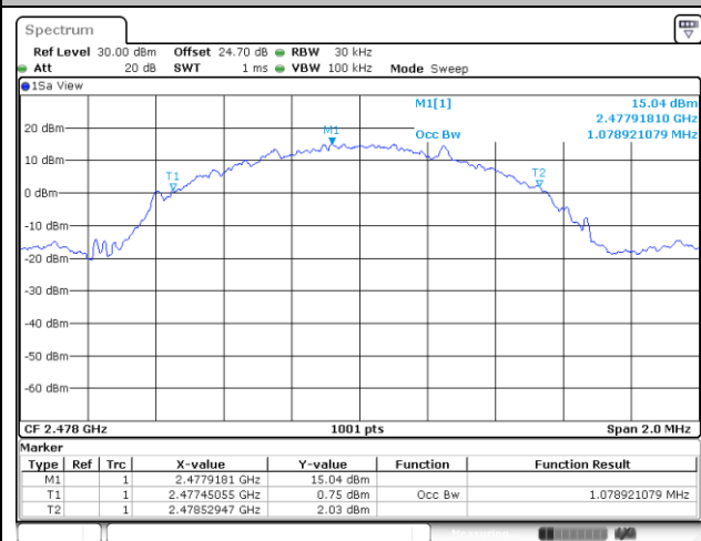
99% Occupied Bandwidth Plot on Channel 76
