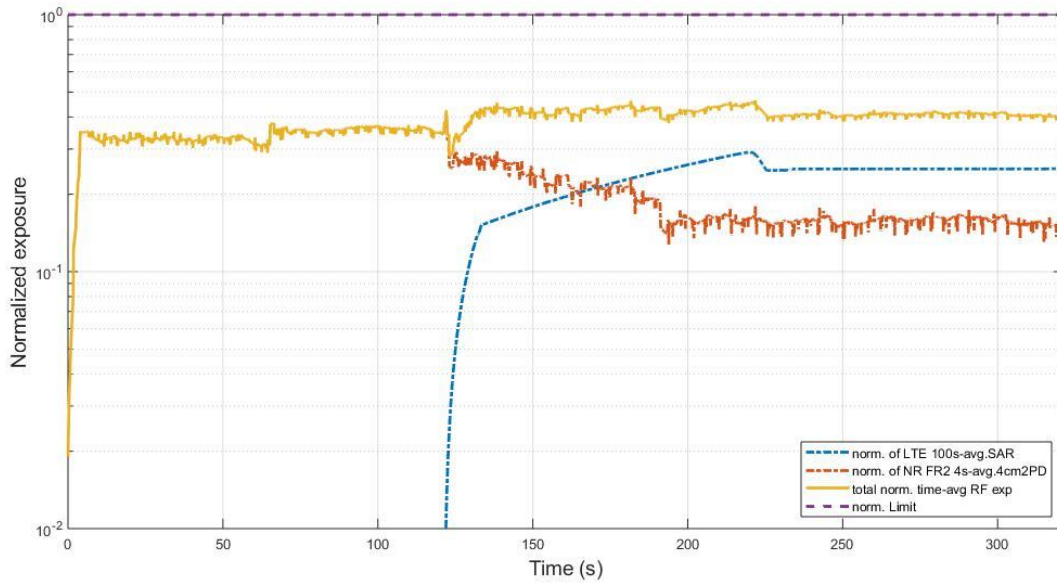
Figure 7.5-2 Total normalized time-average RF exposure in F_TC04
