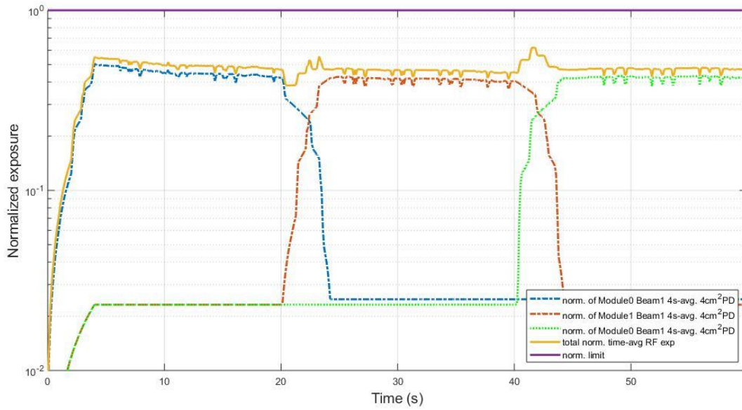
Figure 7.7-2 Total normalized time-average RF exposure
