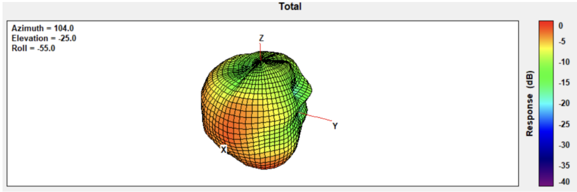
ANT4 Frequency 5180 MHz
