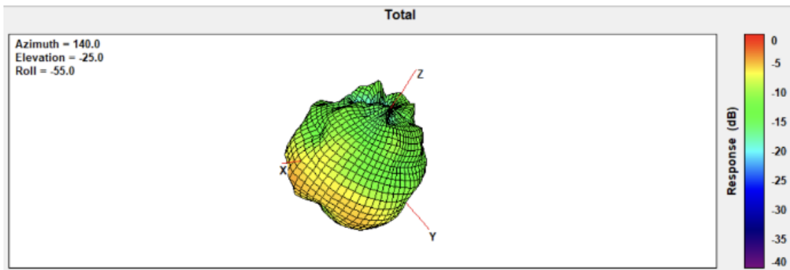
ANT4 Frequency 5500 MHz
