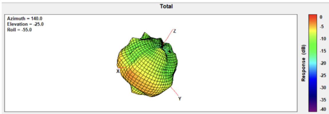
ANT4 Frequency 6175 MHz
