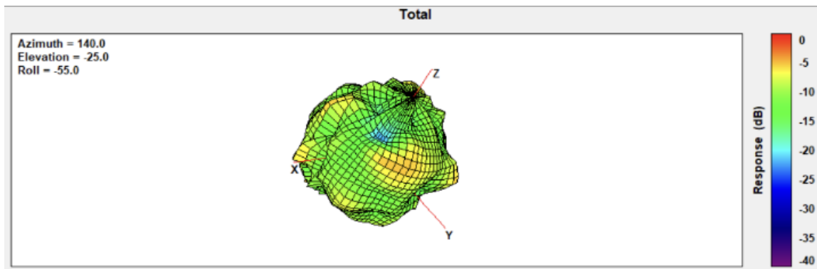
ANT4 Frequency 6475 MHz
