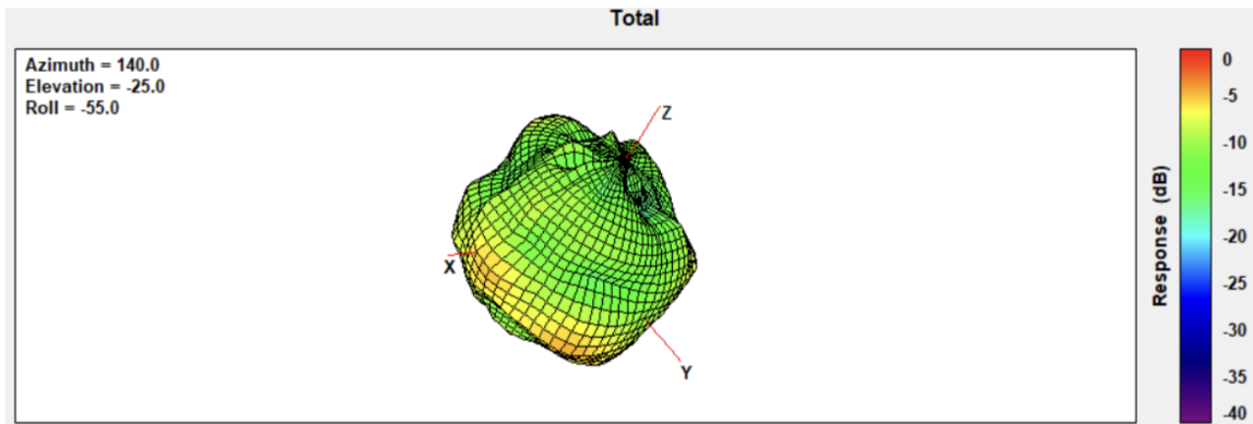
ANT4 Frequency 5280 MHz
