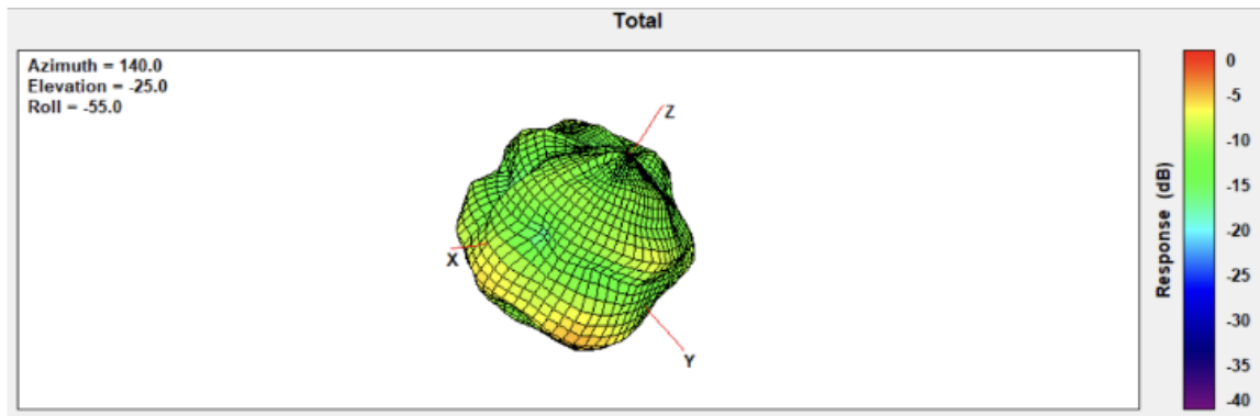
ANT4 Frequency 5500 MHz
