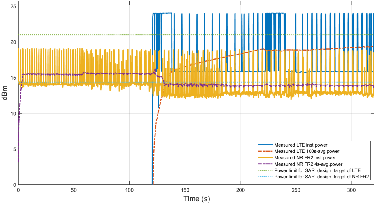
Figure 7.5-1 Conducted power of LTE B2 and radiated EIRP of FR2 n260 in EN-DC max power
