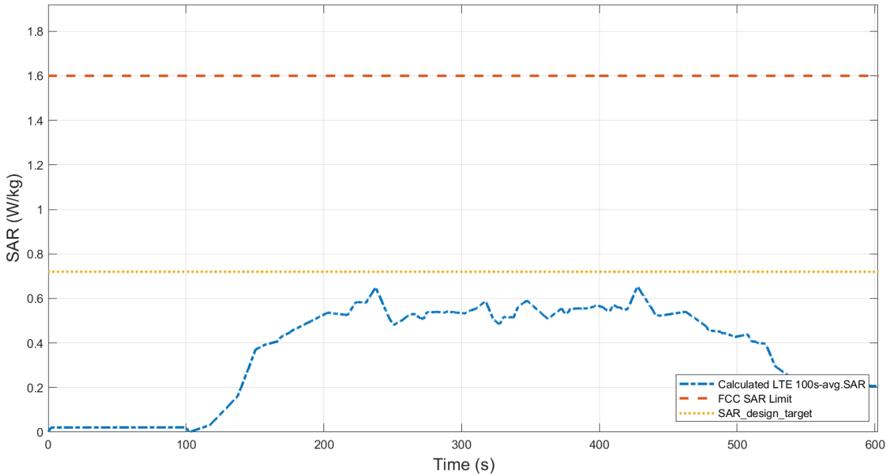
Figure 6.3-10 Total time-averaged SAR
