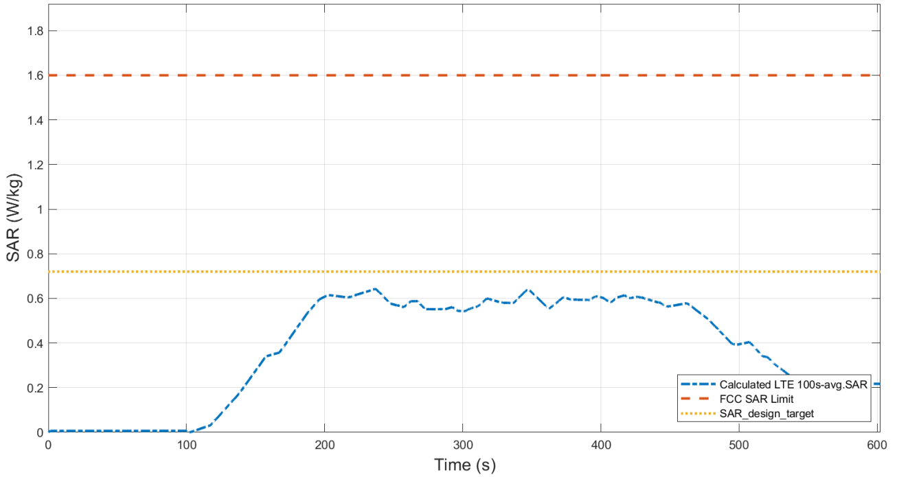
Figure 6.3-12 Total time-averaged SAR
