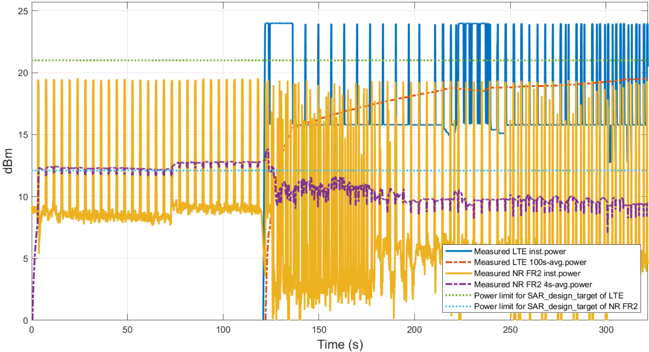
Figure 7.8-1 Conducted power of LTE B2 and radiated EIRP of FR2 n261 in EN-DC max power
