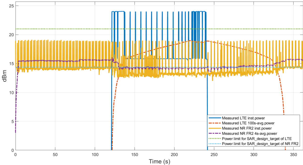
Figure 7.6-1 Conducted power of LTE B2 and radiated EIRP of FR2 n260 in EN-DC max power case
