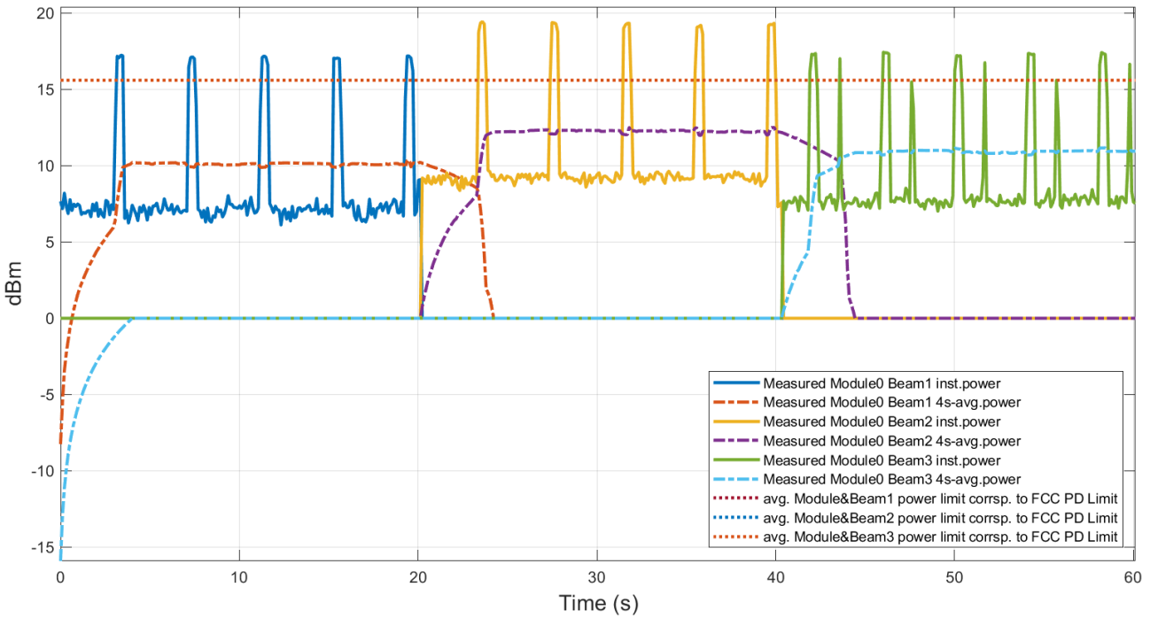
Figure 7.10-1 Measured radiated EIRP of FR2 n260 in mmWave Module beam change case F_TC09
