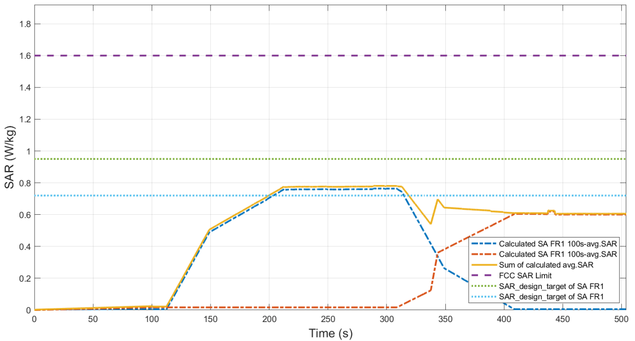
Figure 6.4-2 Total time-averaged SAR
