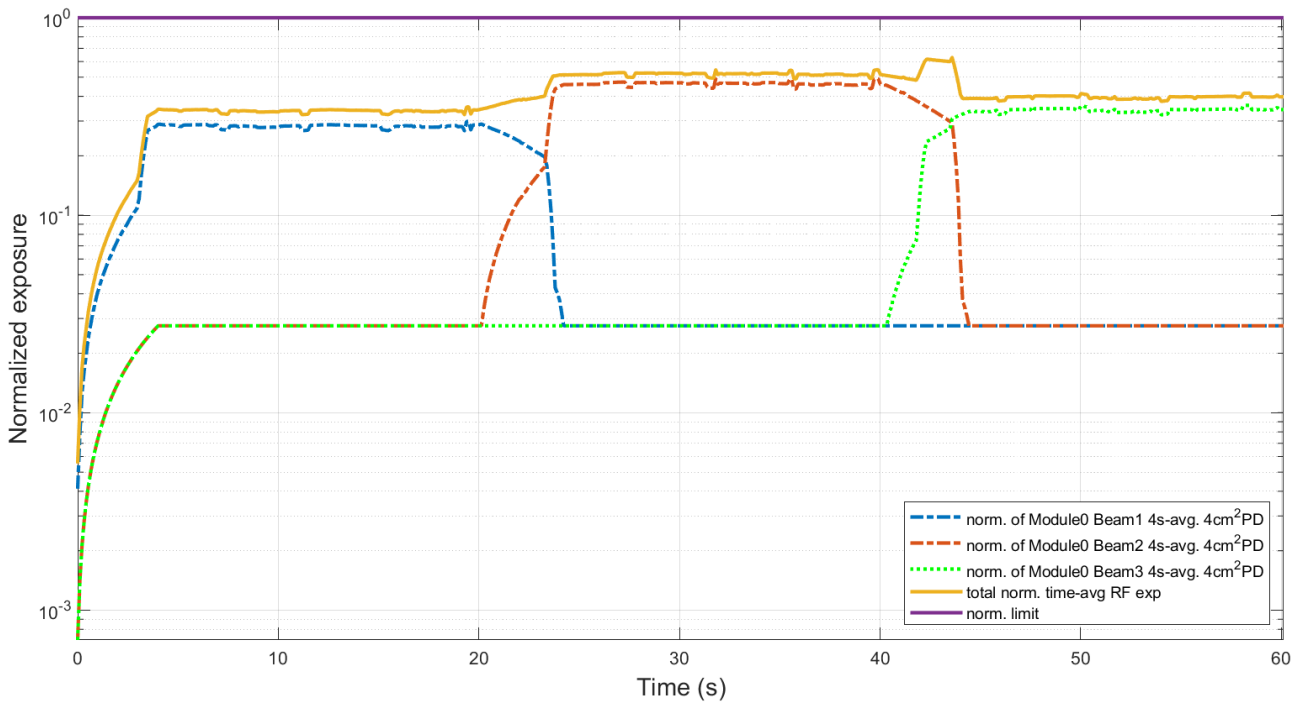
Figure 7.10-2 Total normalized time-average RF exposure
