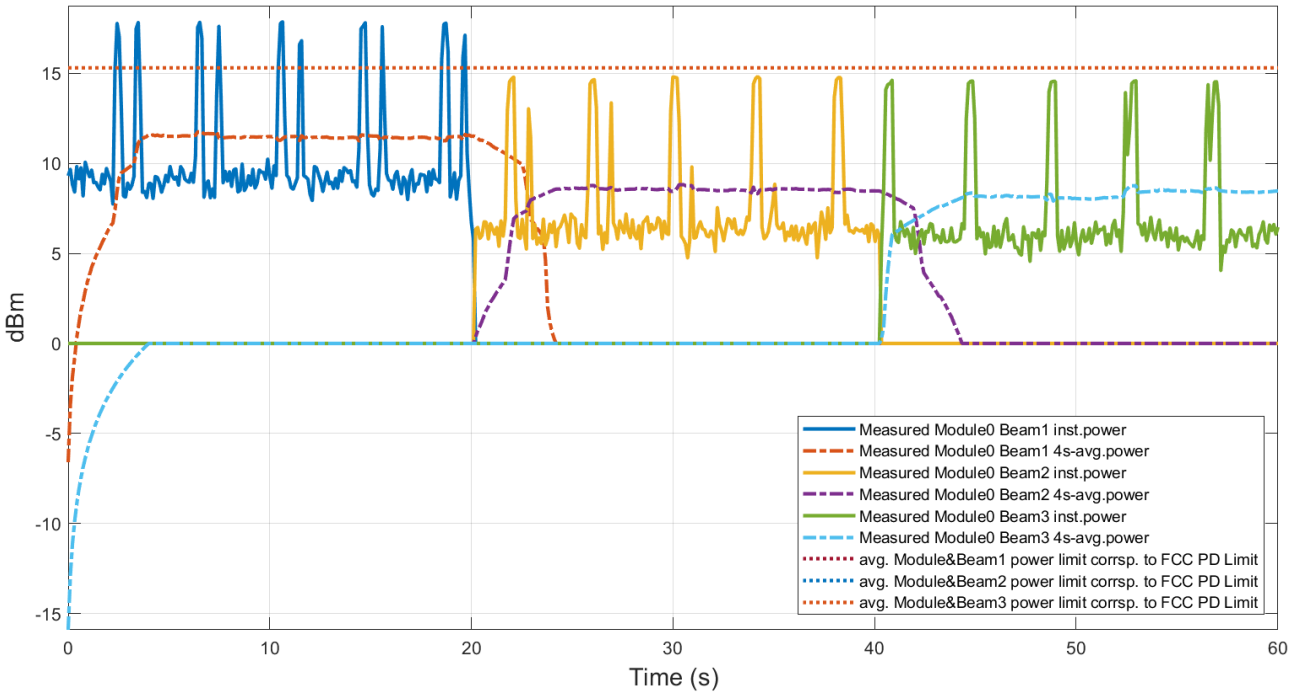
Figure 7.4-1 Measured radiated EIRP of FR2 n258 in mmWave Module beam change case F_TC03
