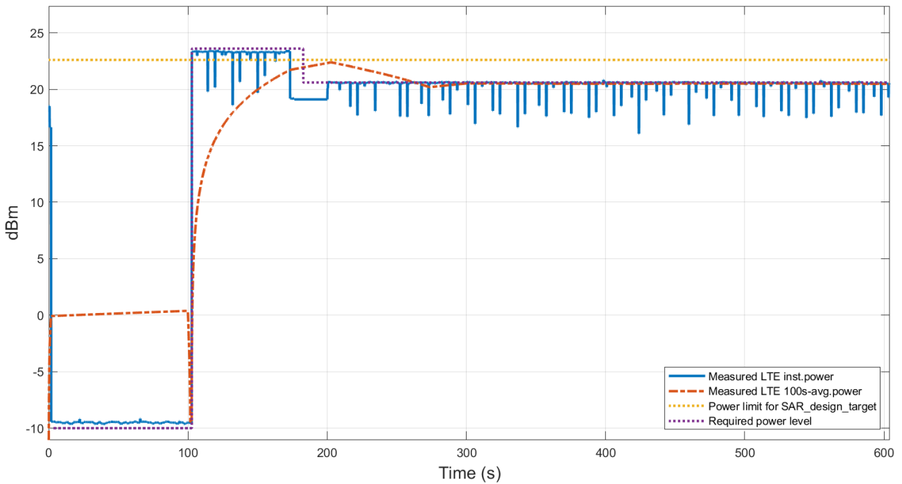
Figure 6.3-3 Time-average conducted power
