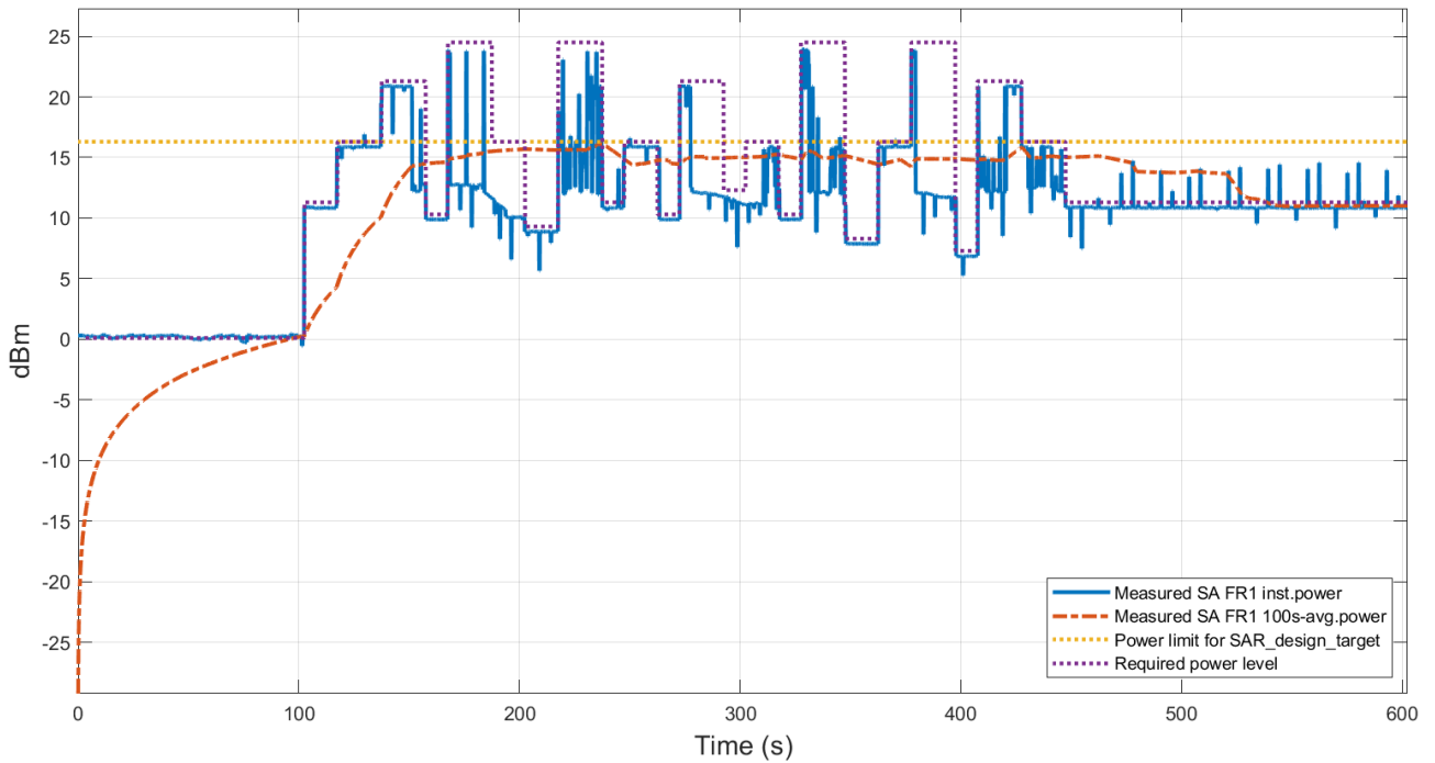
Figure 6.3-13 Conducted Tx power
