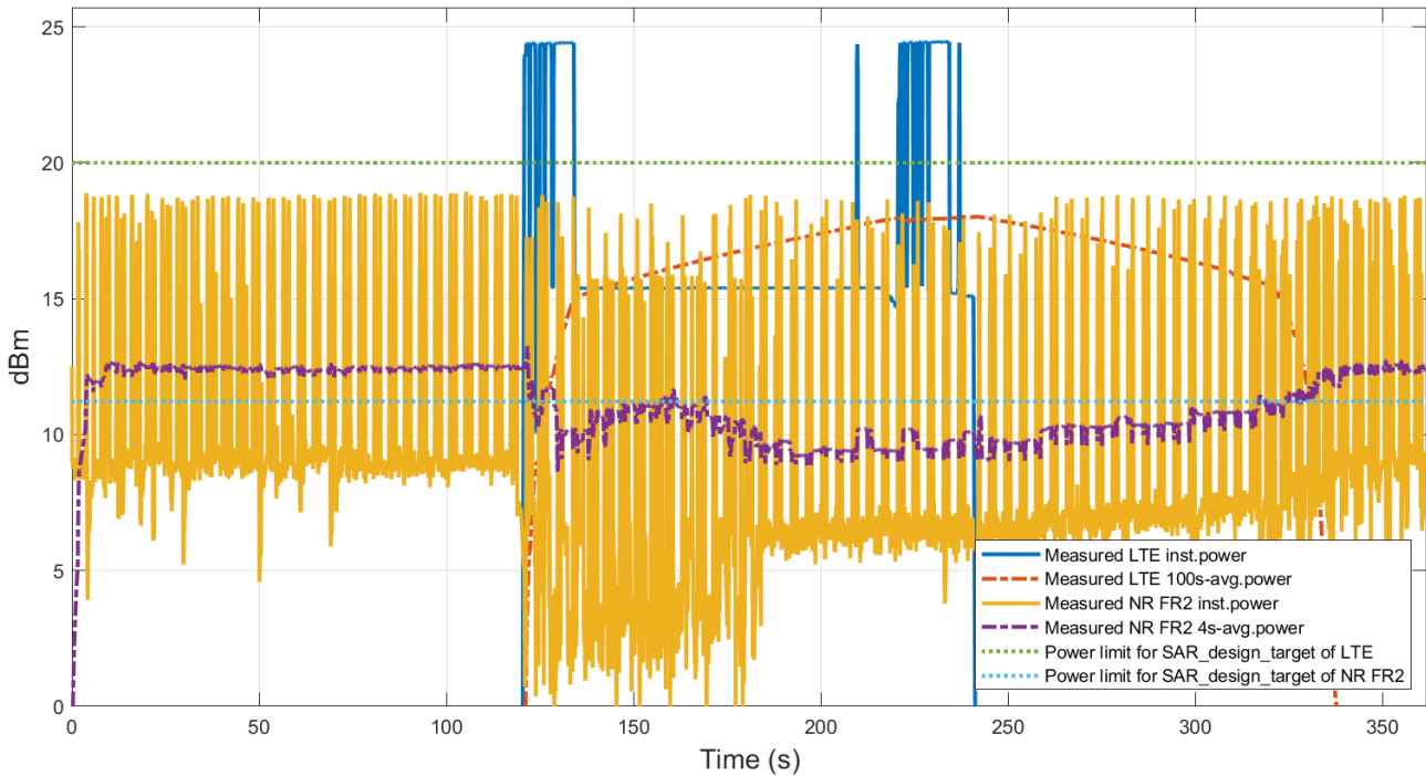
Figure 7.9-1 Conducted power of LTE B2 and radiated EIRP of FR2 n261 in EN-DC max power case
