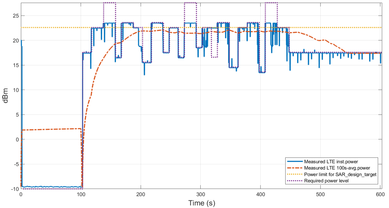
Figure 6.3-11 Conducted Tx power
