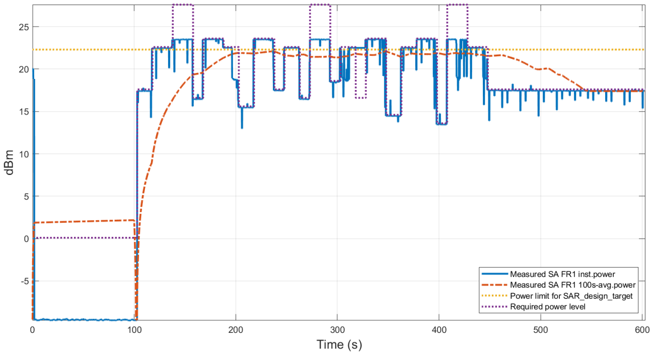
Figure 6.3-15 Conducted Tx power
