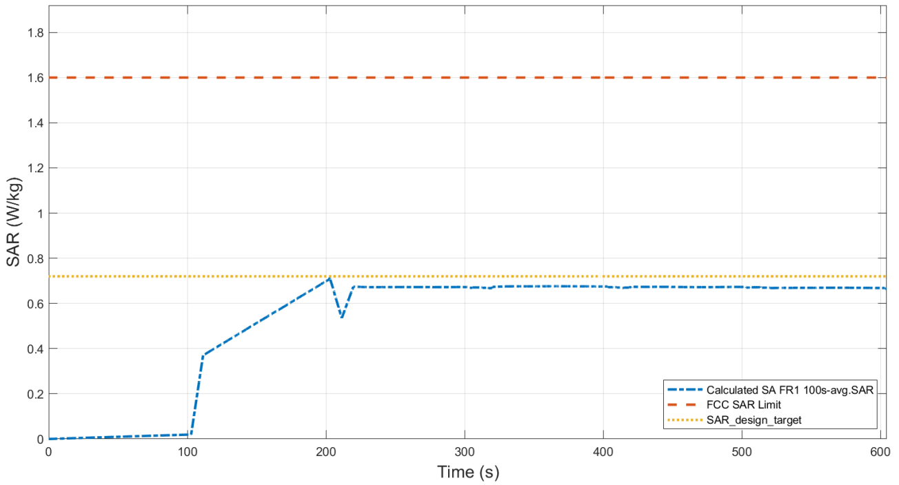
Figure 6.3-6 Total time-averaged SAR
