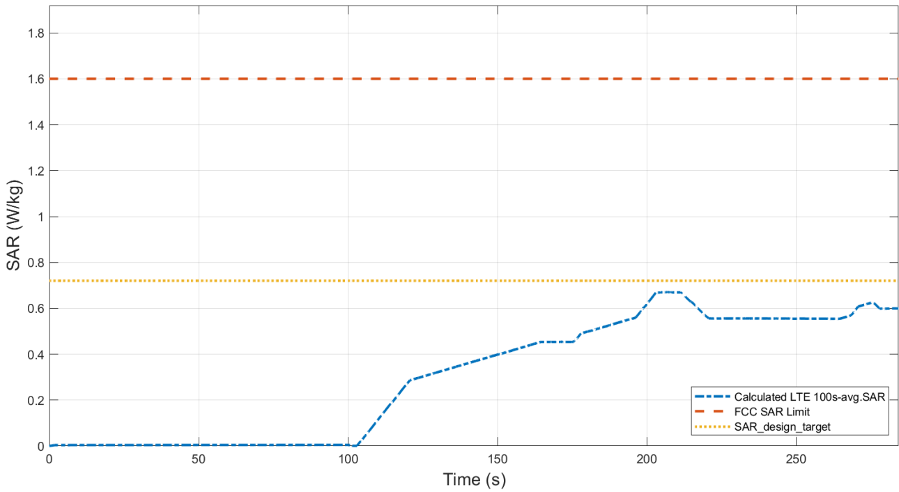
Figure 6.7-2 Total time-averaged SAR
