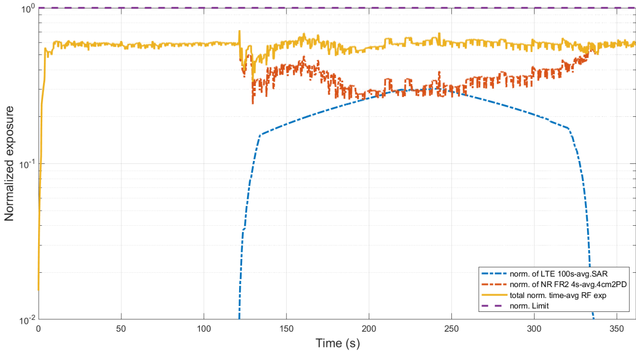
Figure 7.9-2 Total normalized time-average RF exposure in F_TC08
