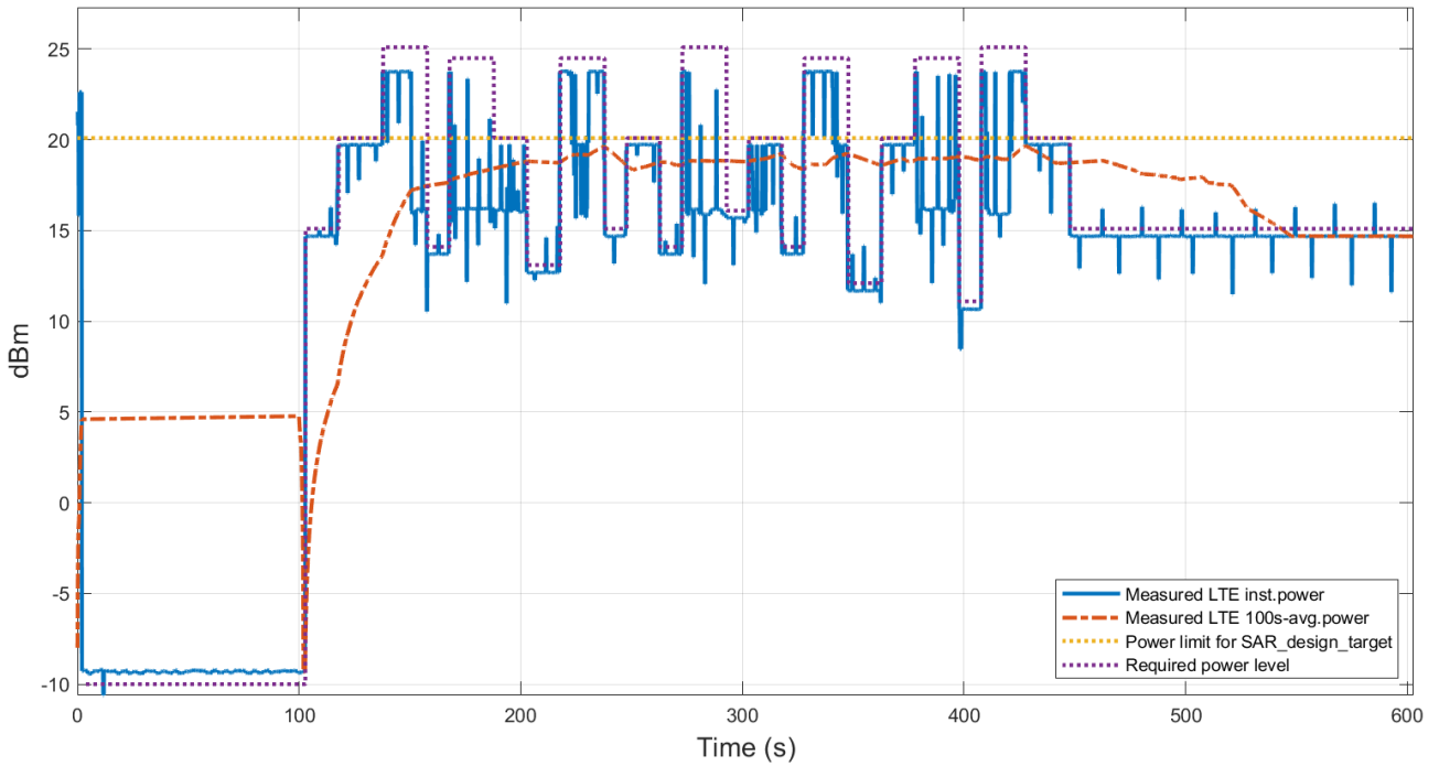
Figure 6.3-9 Conducted Tx power
