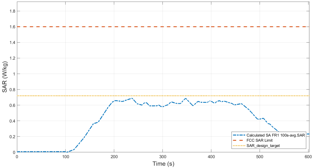
Figure 6.3-16 Total time-averaged SAR
