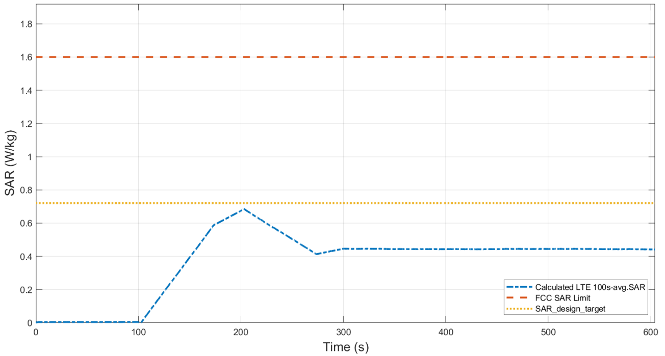
Figure 6.3-4 Total time-averaged SAR
