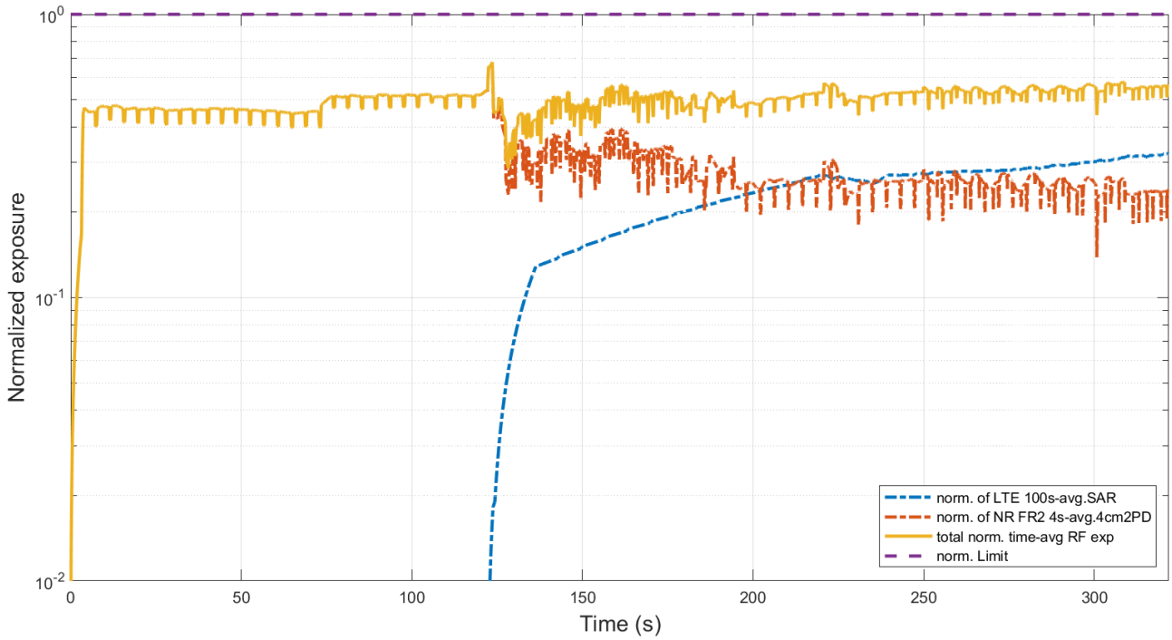
Figure 7.8-2 Total normalized time-average RF exposure in F_TC07
