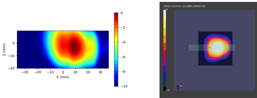
Figure 2-3 Simulated (left) and measured (right) averaged PD distribution for the following configuration: Band n260, MID Channel, Beam ID 0, H polarization, Plane-A Module, plotted on the surface S5 (top) with 10mm separation distance to the DUT.
