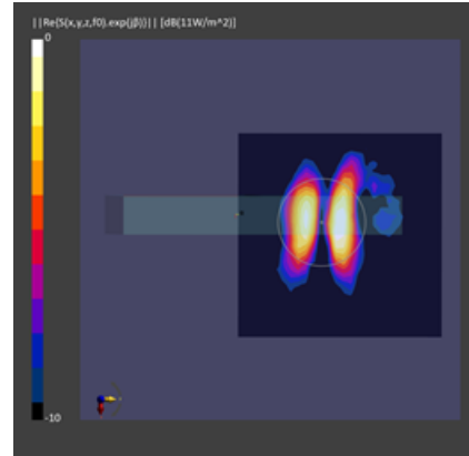
Figure 2-4 Simulated (left) and measured (right) PD distribution for the following configuration: Band n260, MID Channel, Beam ID 1, V polarization, Plane-A Module, plotted on the surface S5 (top) with 10mm separation distance to the DUT.
