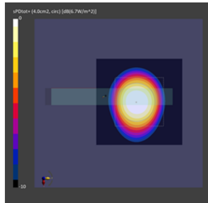
Figure 2-21 Simulated (left) and measured (right) averaged PD distribution for the following configuration: Band n261, MID Channel, Beam ID 2, H polarization, Plane-A Module, plotted on the surface S5 (top) with 10mm separation distance to the DUT.
