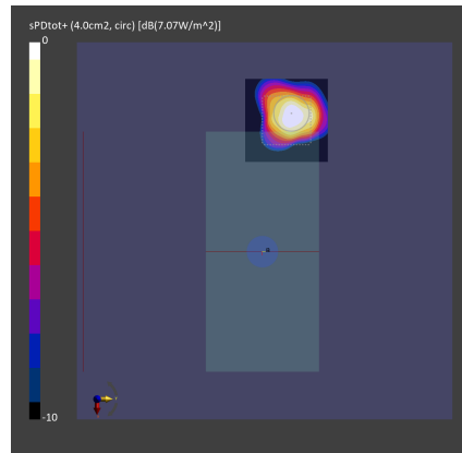
Figure 2-12 Simulated (left) and measured (right) PD distribution for the following configuration: Band n260, MID Channel, Beam ID 1, H+V polarization, Plane-A Module, plotted on the surface S1 (Front) with 2mm separation distance to the DUT.
