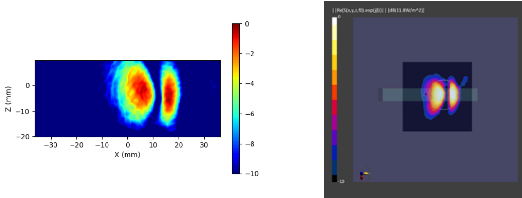
Figure 2-2 Simulated (left) and measured (right) PD distribution for the following configuration: Band n260, MID Channel, Beam ID 0, H polarization, Plane-A Module, plotted on the surface S5 (top) with 10mm separation distance to the DUT.
