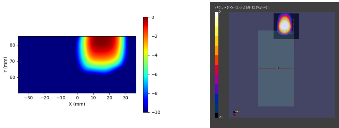
Figure 2-31 Simulated (left) and measured (right) averaged PD distribution for the following configuration: Band n261, MID Channel, Beam ID 3, H+V polarization, Plane-A Module, plotted on the surface S1 (Front) with 2mm separation distance to the DUT.
