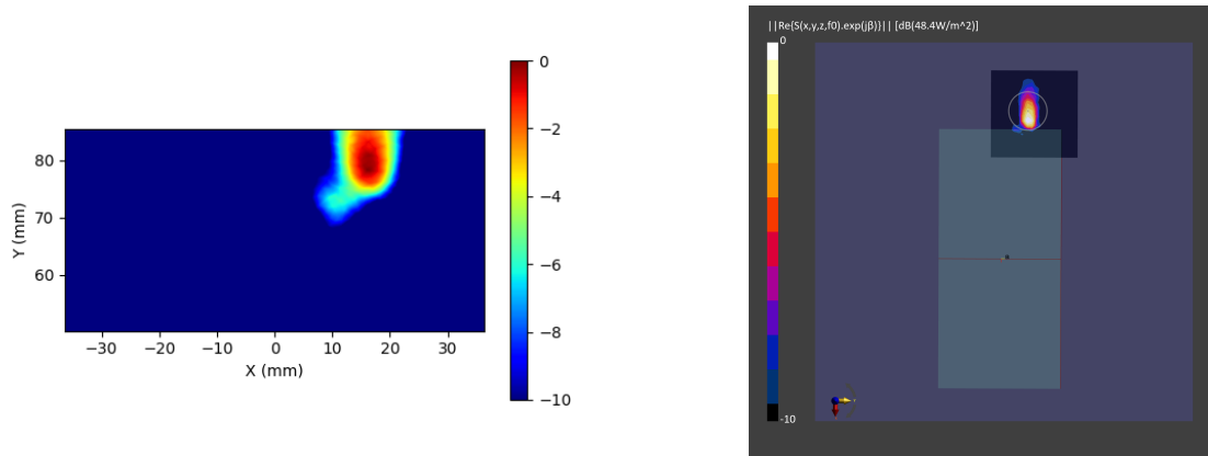
Figure 2-30 Simulated (left) and measured (right) PD distribution for the following configuration: Band n261, MID Channel, Beam ID 3, H+V polarization, Plane-A Module, plotted on the surface S1 (Front) with 2mm separation distance to the DUT.
