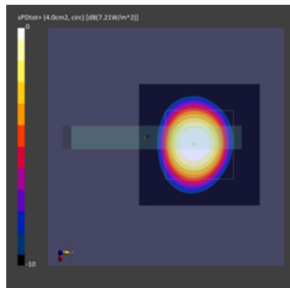
Figure 2-23 Simulated (left) and measured (right) averaged PD distribution for the following configuration: Band n261, MID Channel, Beam ID 3, V polarization, Plane-A Module, plotted on the surface S 5 (top) with 10mm separation distance to the DUT.
