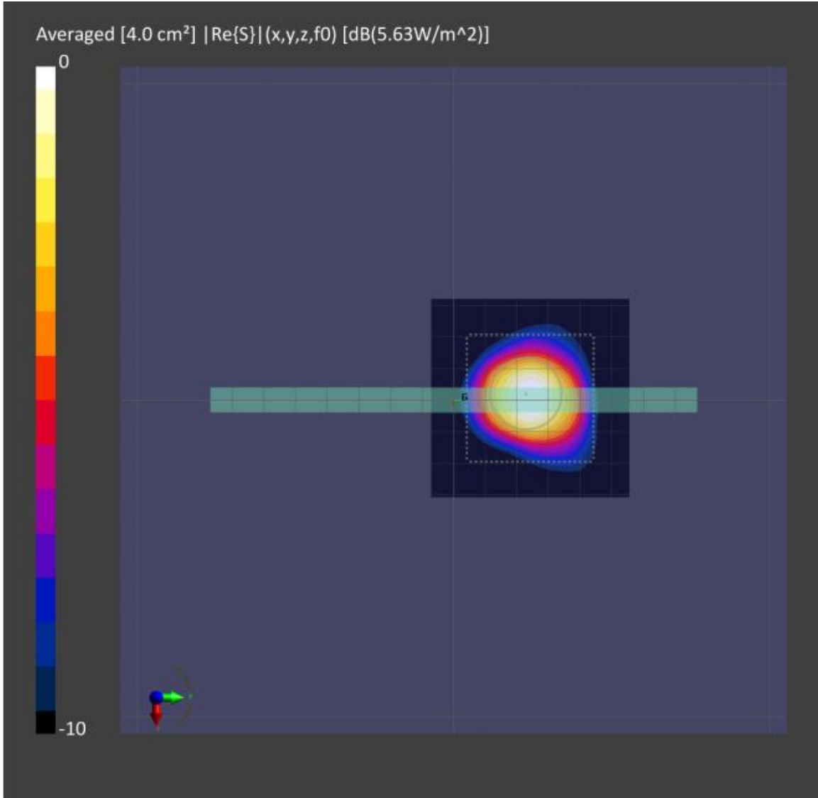
Figure 7-2: 4cm2-averaged power density distribution measured at input.power.limit of 4.118 dBm on the Right Side surface for n261 beam 22
