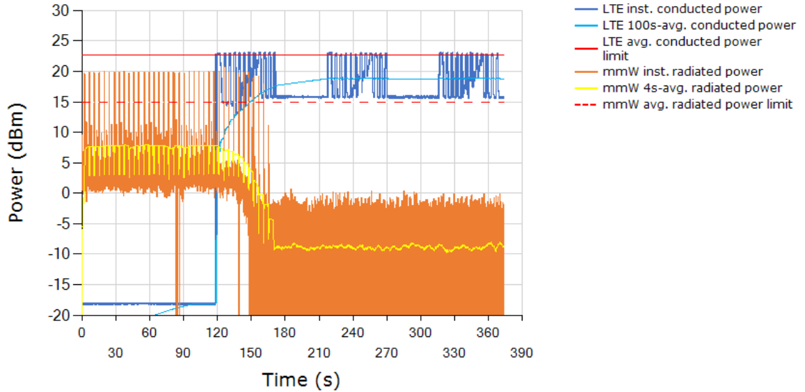
LTE and mmW Instantaneous and Time-averaged TX Power Tech: LTE, Band 66 / Tech: NR5G MMW, Band n261
