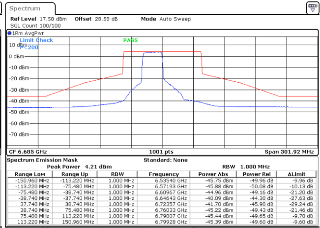
Plot on Channel 6685 MHz
