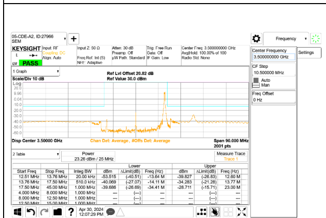
5G NR n77 25MHz BPSK Middle Channel RB1-64, ID:27966
