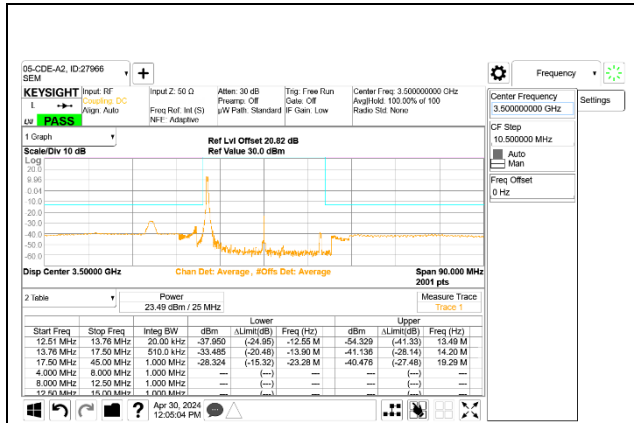
5G NR n77 25MHz BPSK Middle Channel RB1-0, ID:27966
