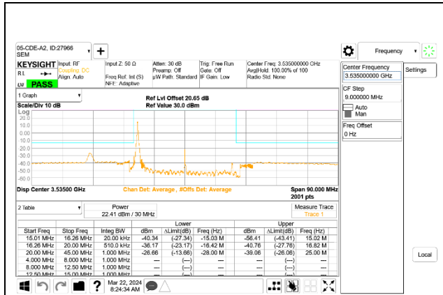
5G NR n77 30MHz BPSK High Channel RB1-0, ID:27966
