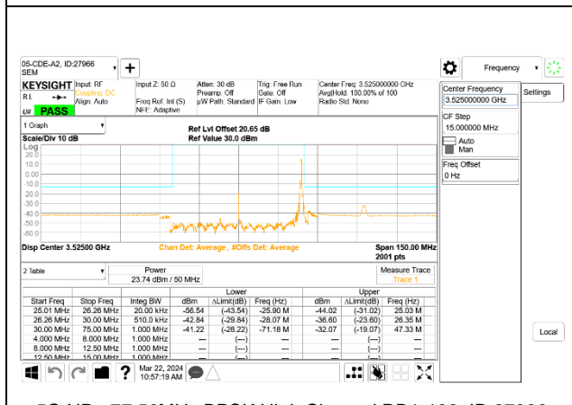
5G NR n77 50MHz BPSK High Channel RB1-132, ID:27966
