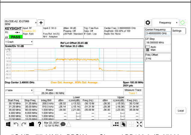
5G NR n77 60MHz BPSK Low Channel RB162-0, ID:27966
