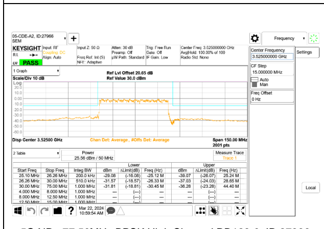
5G NR n77 50MHz BPSK High Channel RB128-0, ID:27966
