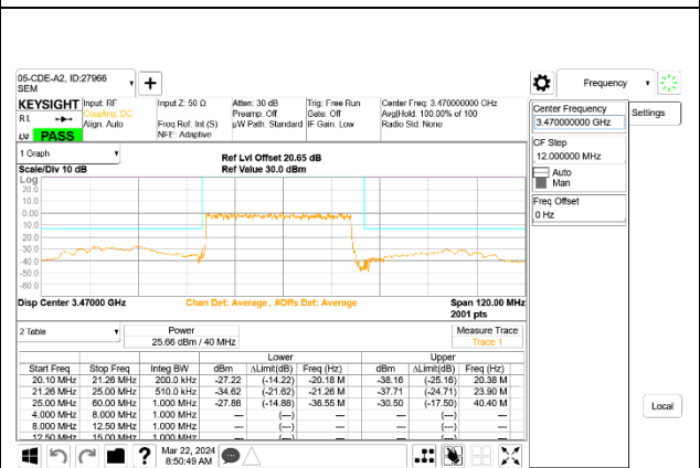
5G NR n77 40MHz BPSK Low Channel RB100-0, ID:27966
