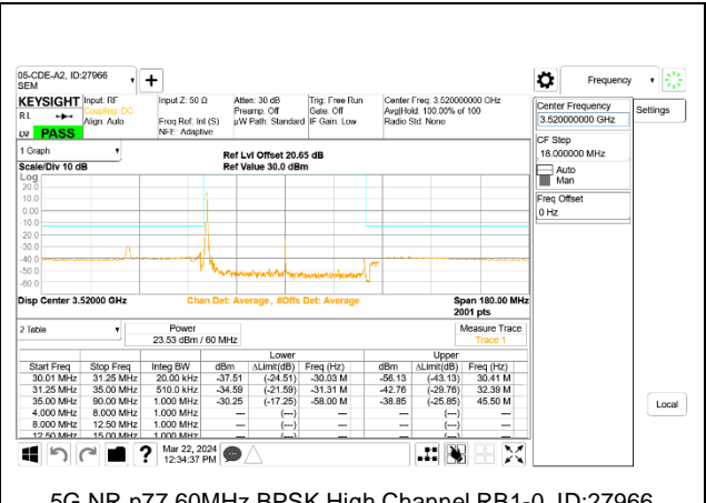
5G NR n77 60MHz BPSK High Channel RB1-0, ID:27966
