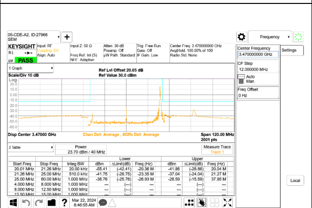
5G NR n77 40MHz BPSK Low Channel RB1-105, ID:27966
