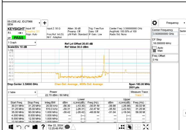
5G NR n77 60MHz BPSK Middle Channel RB1-161, ID:27966
