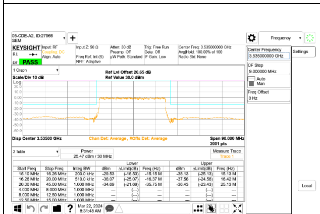
5G NR n77 30MHz BPSK High Channel RB75-0, ID:27966
