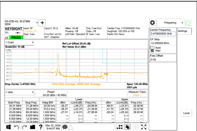
5G NR n77 40MHz BPSK Low Channel RB1-0, ID:27966
