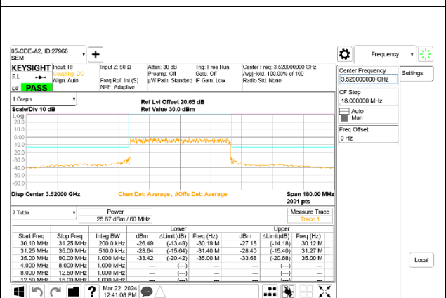
5G NR n77 60MHz BPSK High Channel RB162-0, ID:27966
