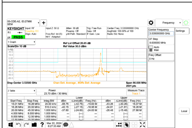
5G NR n77 30MHz BPSK High Channel RB1-77, ID:27966
