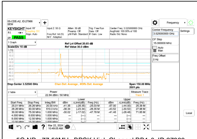
5G NR n77 50MHz BPSK High Channel RB1-0, ID:27966
