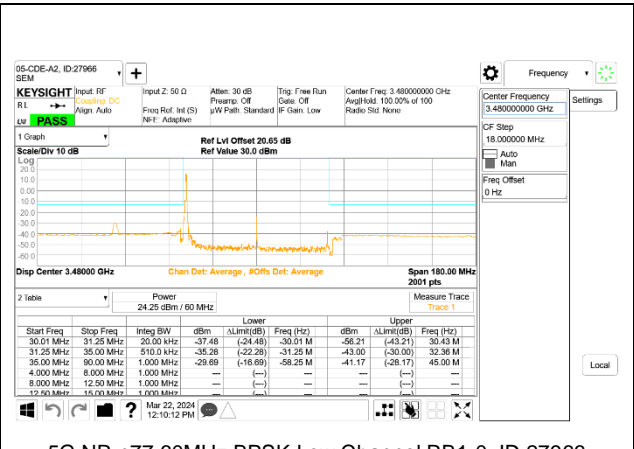
5G NR n77 60MHz BPSK Low Channel RB1-0, ID:27966
