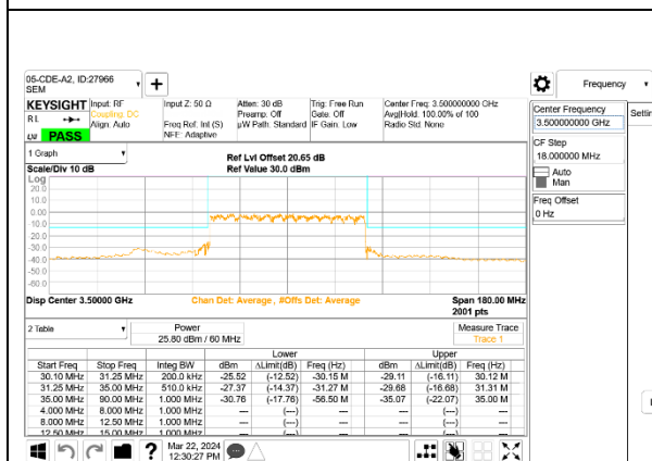
5G NR n77 60MHz BPSK Middle Channel RB162-0, ID:27966
