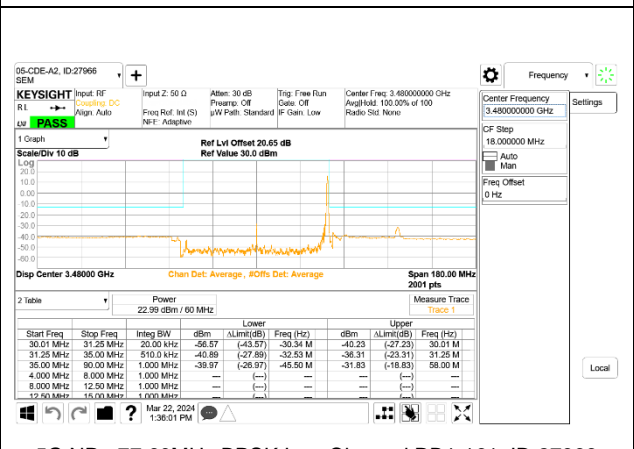
5G NR n77 60MHz BPSK Low Channel RB1-161, ID:27966
