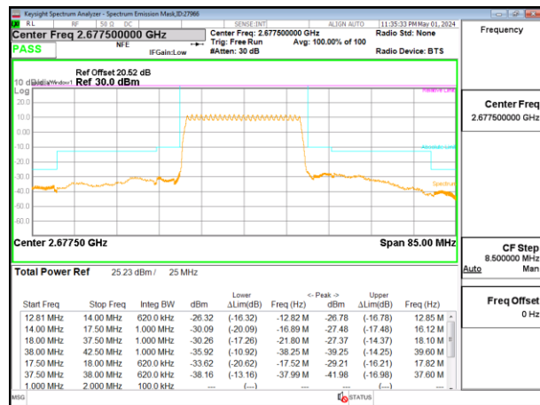
5G NR n41 25MHz BPSK High Channel RB64-0, ID:27966
