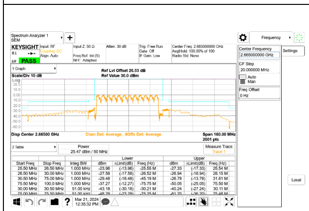
5G NR n41 50MHz BPSK High Channel RB128-0, ID:27966
