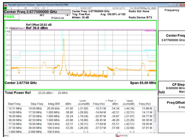
5G NR n41 25MHz BPSK High Channel RB1-0, ID:27966
