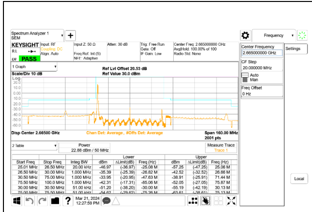
5G NR n41 50MHz BPSK High Channel RB1-0, ID:27966
