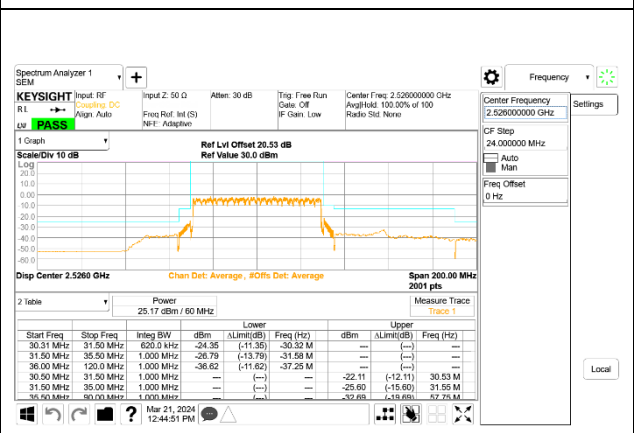
5G NR n41 60MHz BPSK Low Channel RB162-0, ID:27966
