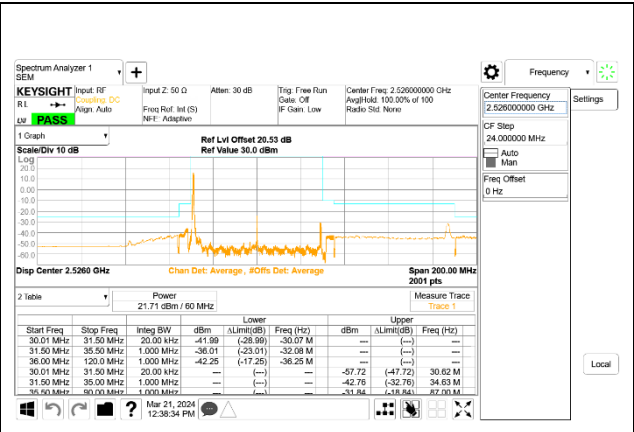
5G NR n41 60MHz BPSK Low Channel RB1-0, ID:27966
