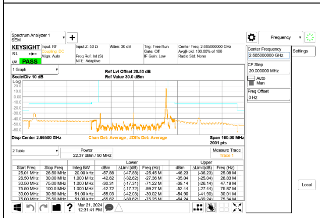
5G NR n41 50MHz BPSK High Channel RB1-132, ID:27966
