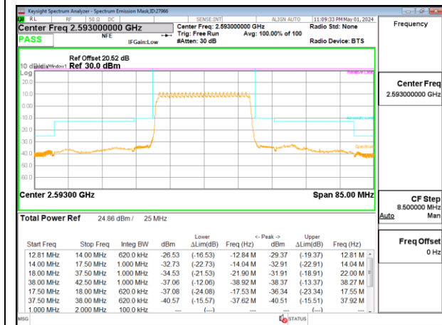
5G NR n41 25MHz BPSK Middle Channel RB64-0, ID:27966
