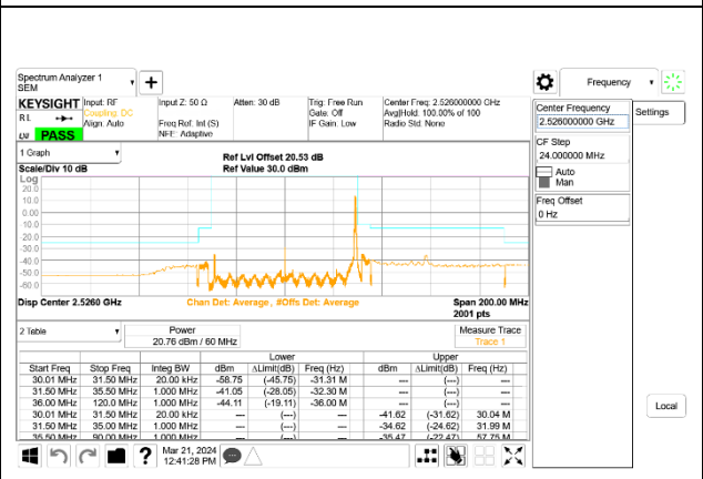
5G NR n41 60MHz BPSK Low Channel RB1-161, ID:27966
