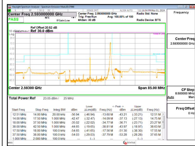
5G NR n41 25MHz BPSK Middle Channel RB1-64, ID:27966
