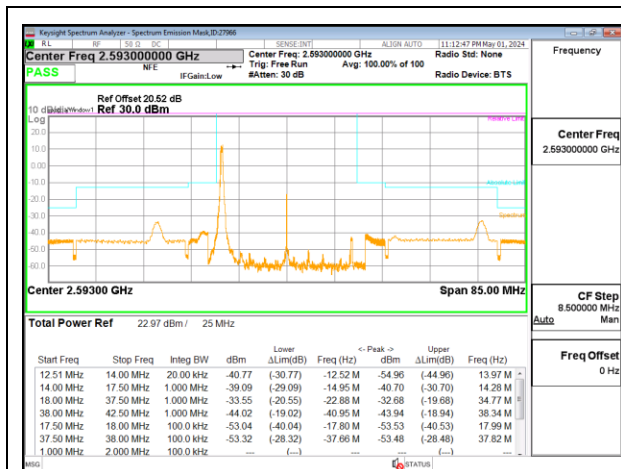
5G NR n41 25MHz BPSK Middle Channel RB1-0, ID:27966
