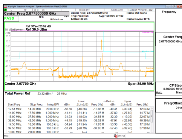
5G NR n41 25MHz BPSK High Channel RB1-64, ID:27966
