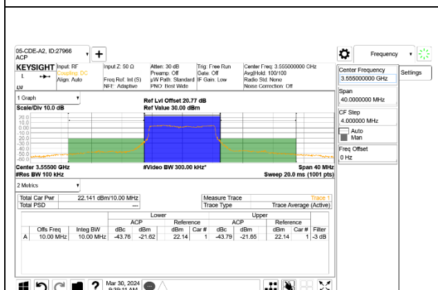
5G NR n48 10MHz BPSK Low Channel RB24-0, ID:27966
