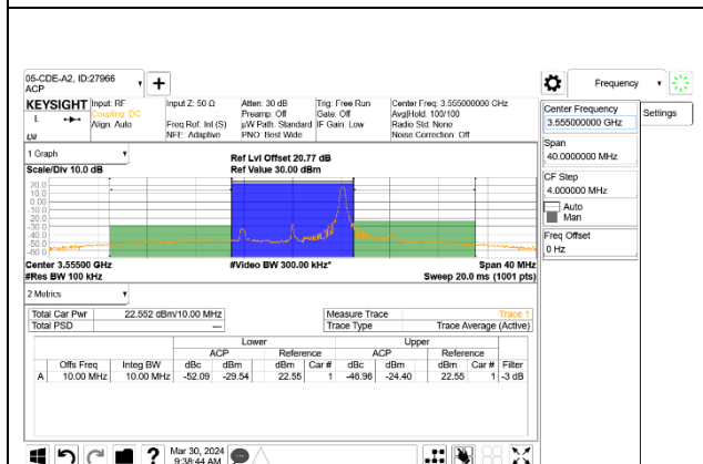
5G NR n48 10MHz BPSK Low Channel RB1-23, ID:27966
