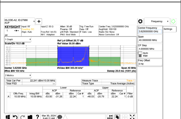
5G NR n48 10MHz BPSK Middle Channel RB1-23, ID:27966
