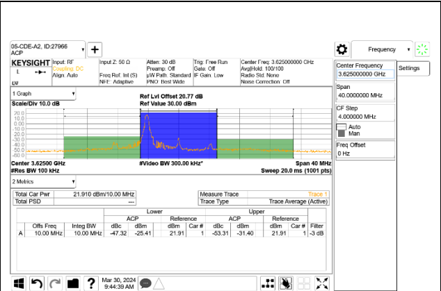
5G NR n48 10MHz BPSK Middle Channel RB1-0, ID:27966
