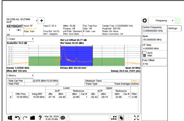
5G NR n48 10MHz BPSK Low Channel RB1-0, ID:27966
