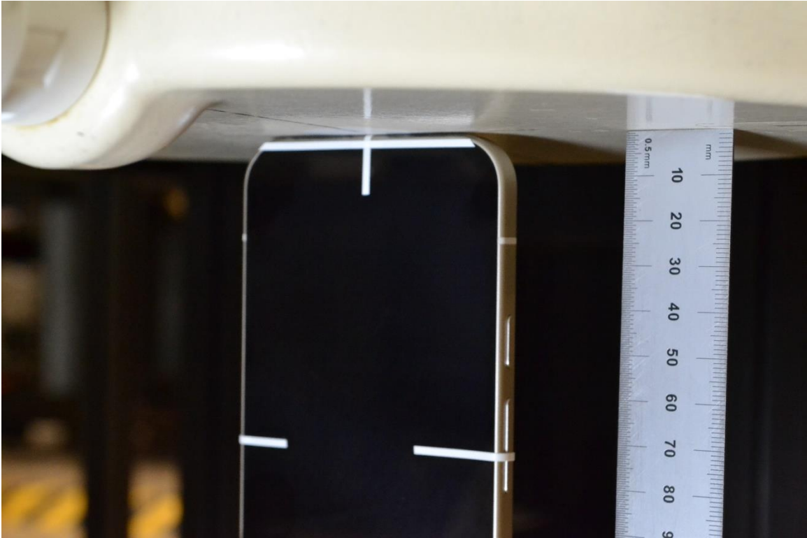
Photograph 23: Top, 0 mm
