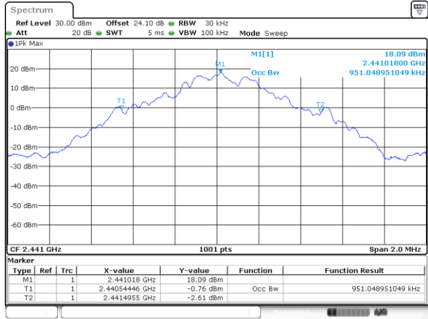
99% Occupied Bandwidth on Channel 39
