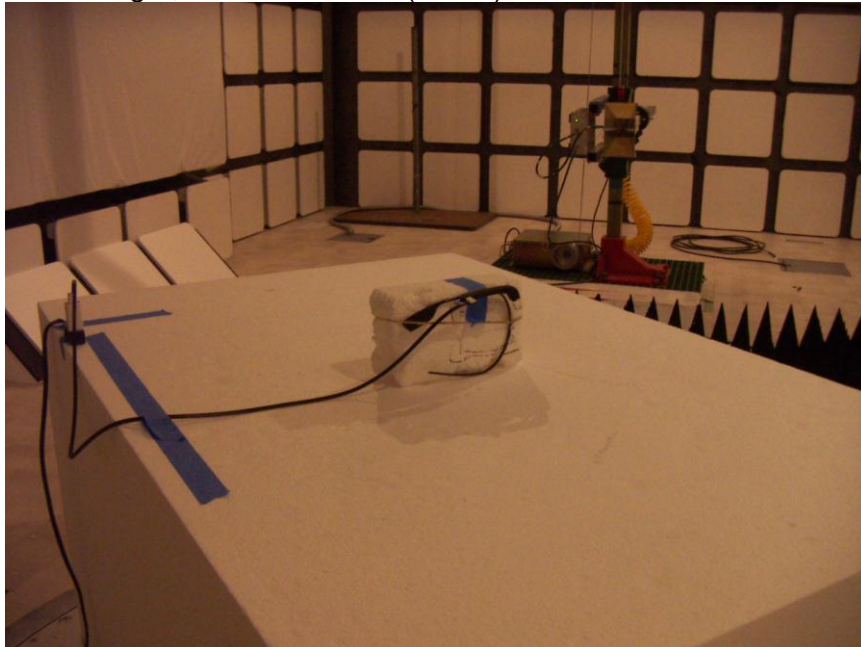
With charger, 1000-6000 MHz (BACK)
