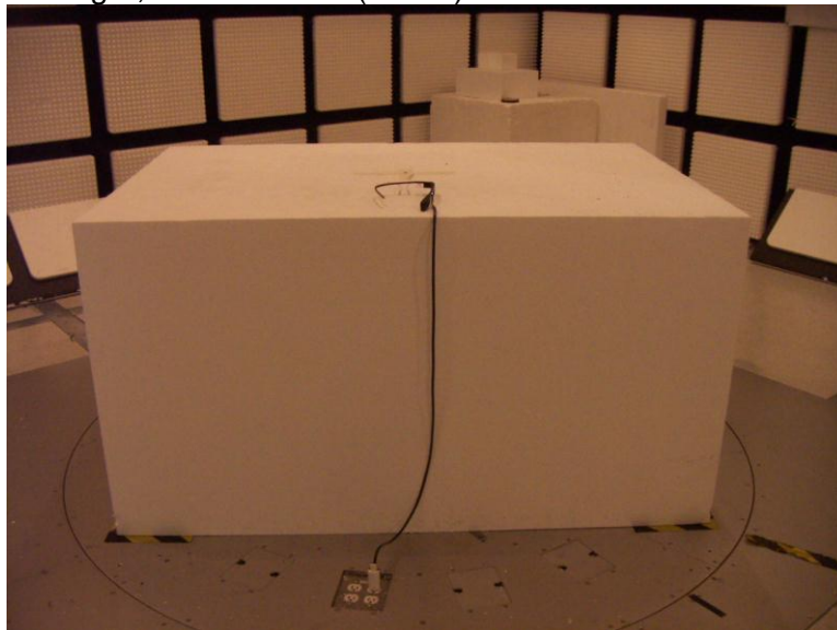
With charger, 30-1000 MHz (BACK)
