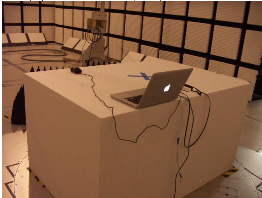
With laptop PC, 1000-6000 MHz (BACK)
