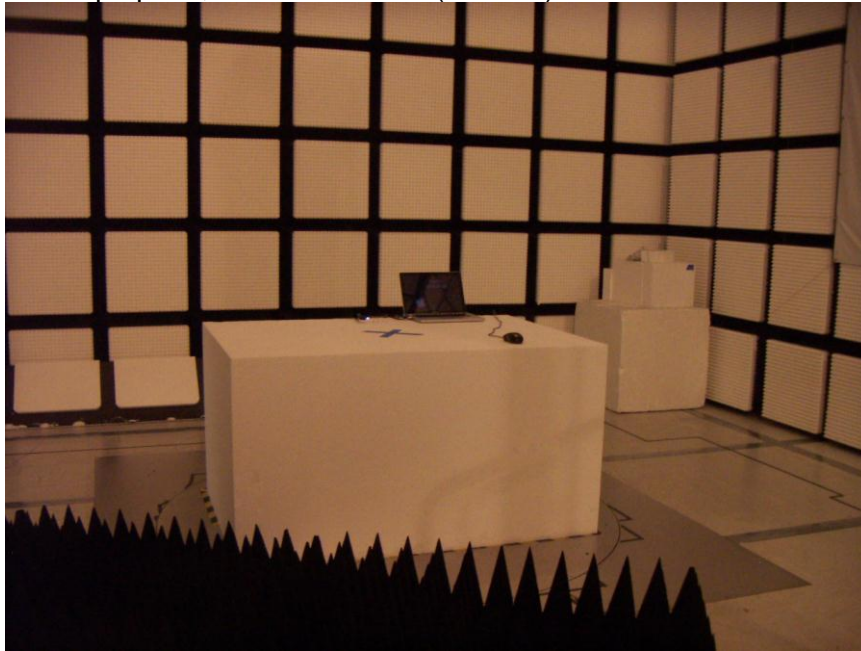
With laptop PC, 1000-6000 MHz (FRONT)
