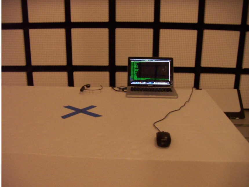
With laptop PC, 30-1000 MHz (FRONT)
