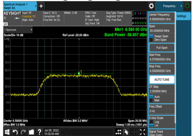
802.11ax_160MHz_6665MHz_AWGN:6590
