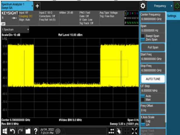
Det Le1_802.11ax_160MHz_CF 6665MHz_6590MHz_-69.33dBm
