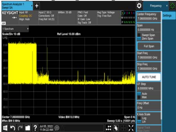
Det Le1_802.11ax_160MHz_CF 6985MHz_7060MHz_-72.18dBm
