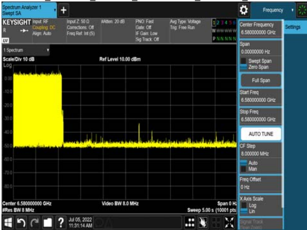
Det Le1_802.11ax_160MHz_CF 6505MHz_6580MHz_-76.29dBm
