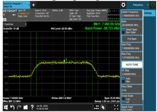
802.11ax_160MHz_6985MHz_AWGN:7060
