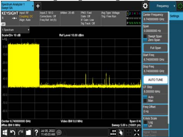
Det Le1_802.11ax_160MHz_CF 6665MHz_6740MHz_-74.02dBm
