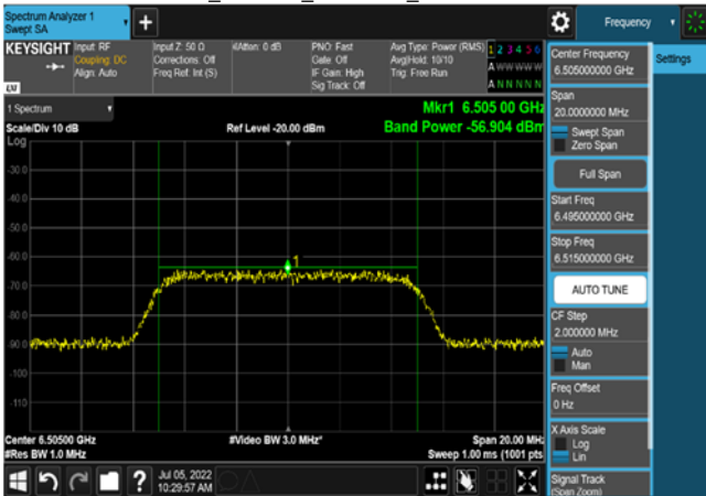
802.11ax_160MHz_6505MHz_AWGN:6505MHz
