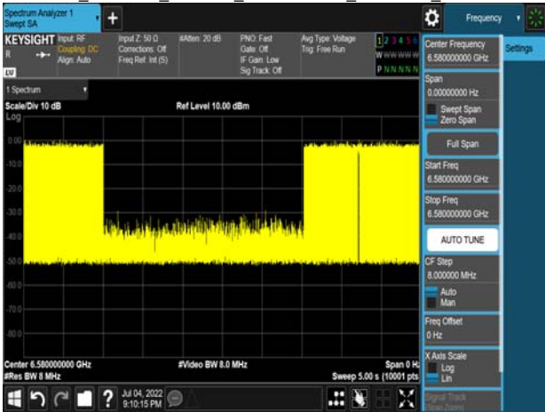
Det Le1_802.11ax_160MHz_CF 6505MHz_6580MHz_-75.29dBm
