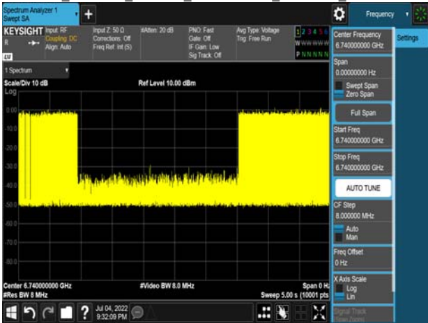
Det Lel_802.11ax_160MHz_CF 6665MHz_6740MHz_-73.02dBm
