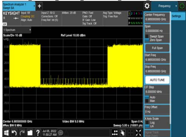
Det Le1_802.11ax_160MHz_CF 6985MHz_6985MHz_-67.35dBm
