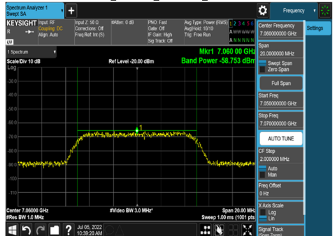
802.11ax_160MHz_6985MHz_AWGN:7060
