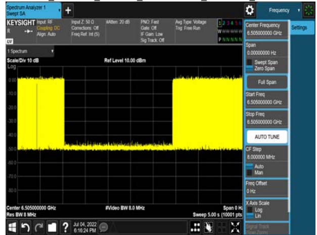
Det Lel_802.11ax_160MHz_CF 6505MHz_6505MHz-69.11dBm
