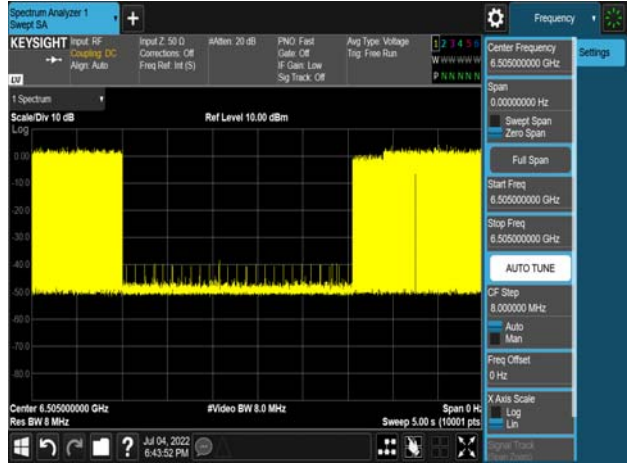
Det Lel_802.11ax_160MHz_CF 6505MHz_6505MHz-70.11dBm
