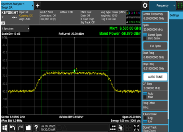
802.11ax_160MHz_6505MHz_AWGN:6505MHz
