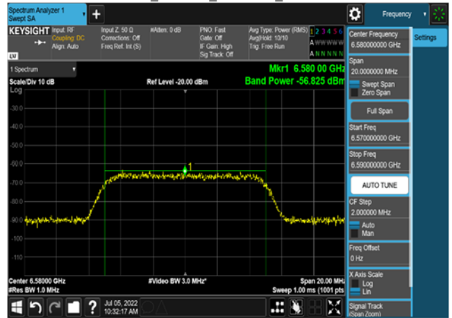
802.11ax_160MHz_6665MHz_AWGN:6590
