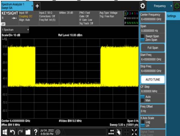
Det Le1_802.11ax_160MHz_CF 6505MHz_6430MHz_-75.17dBm
