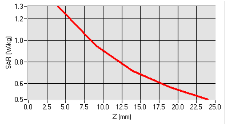
SAR, Z Axis Scan (X = -48, Y = -32)
