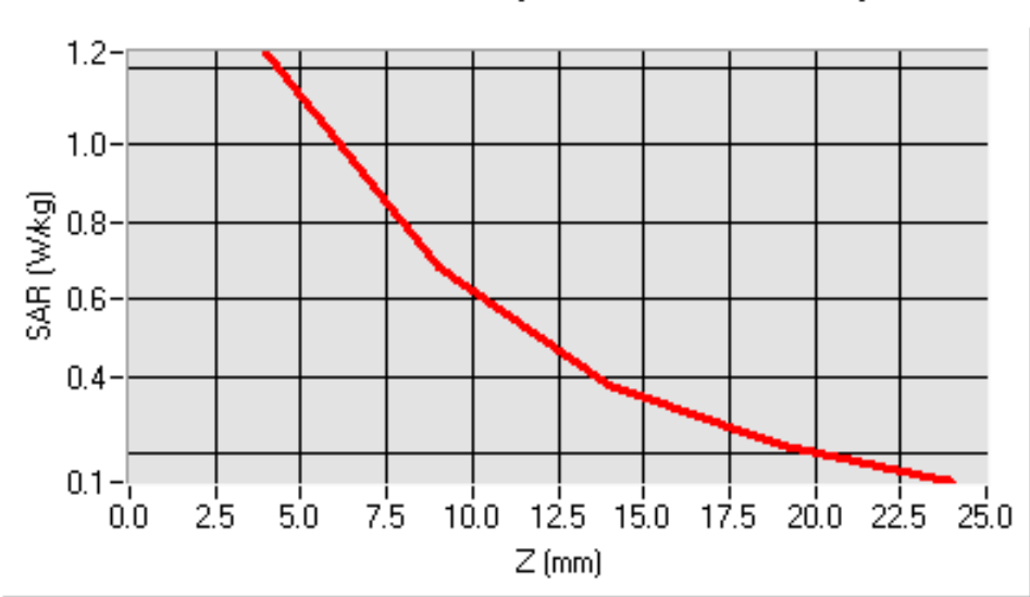
SAR, Z Axis Scan (X = -48, Y = -30)
