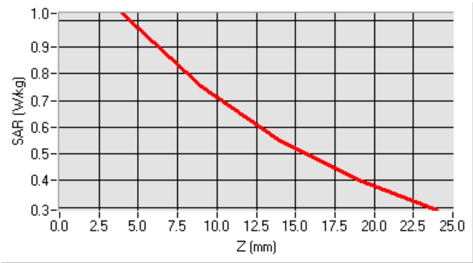
SAR, Z Axis Scan (X = -55, Y = -31)
