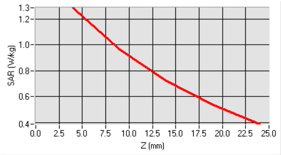
SAR, Z Axis Scan (X = -48, Y = -30)
