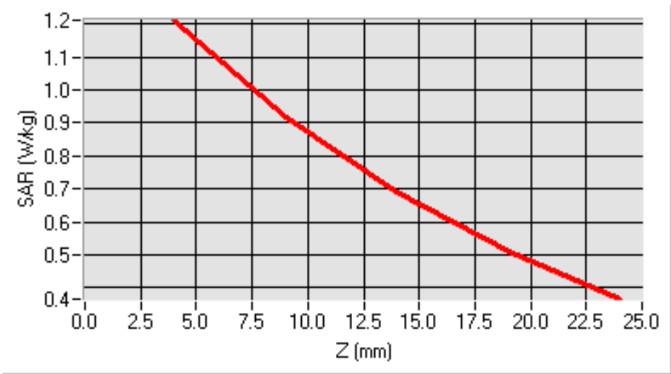
SAR, Z Axis Scan (X = -47, Y = -30)
