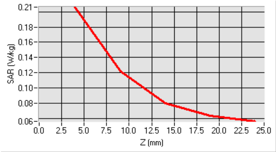
SAR, Z Axis Scan (X = -17, Y = 5)
