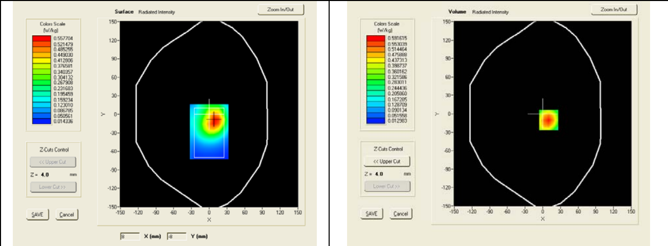
SAR, Z Axis Scan (X = 10, Y = -10)
