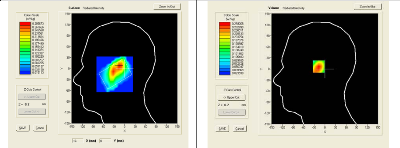
SAR, Z Axis Scan (X = -15, Y = 7)
