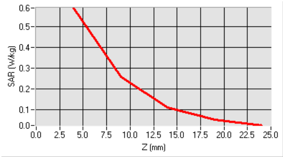
SAR, Z Axis Scan (X = 10, Y = -10)
