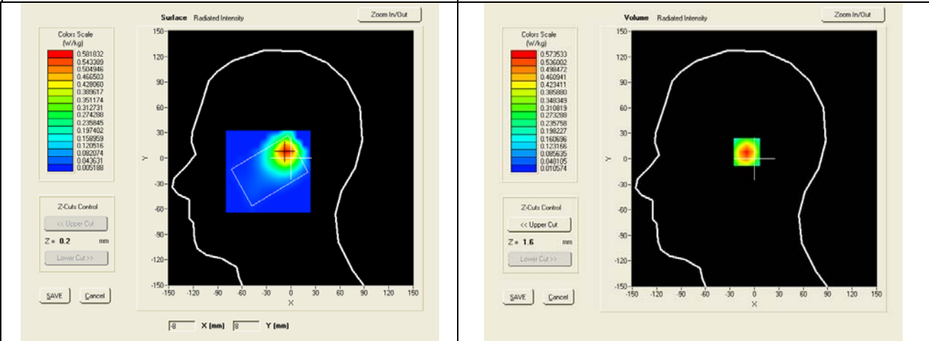
SAR, Z Axis Scan (X = -6, Y = 8)
