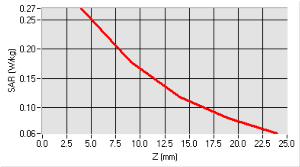
SAR, Z Axis Scan (X = -15, Y = 7)
