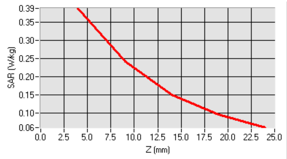
SAR, Z Axis Scan (X = -13, Y = 1)
