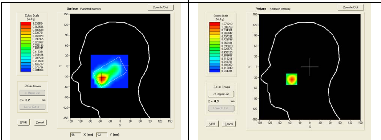
SAR, Z Axis Scan (X = -54, Y = -35)
