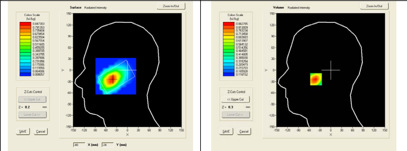
SAR, Z Axis Scan (X = -41, Y = -24)
