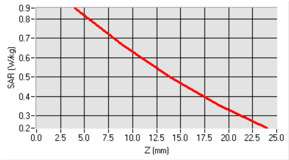
SAR, Z Axis Scan (X = -42, Y = -27)
