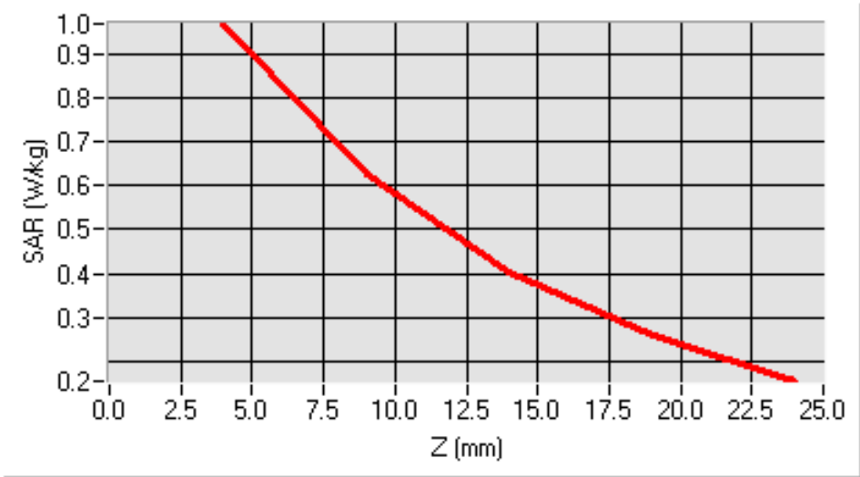
SAR, Z Axis Scan (X = -54, Y = -37)
