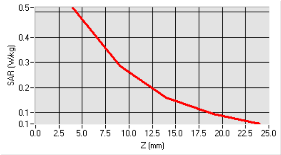
SAR, Z Axis Scan (X = -8, Y = -24)
