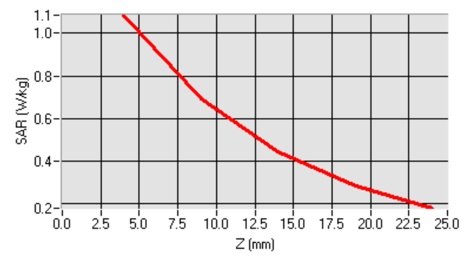
SAR, Z Axis Scan (X = -50, Y = -33)
