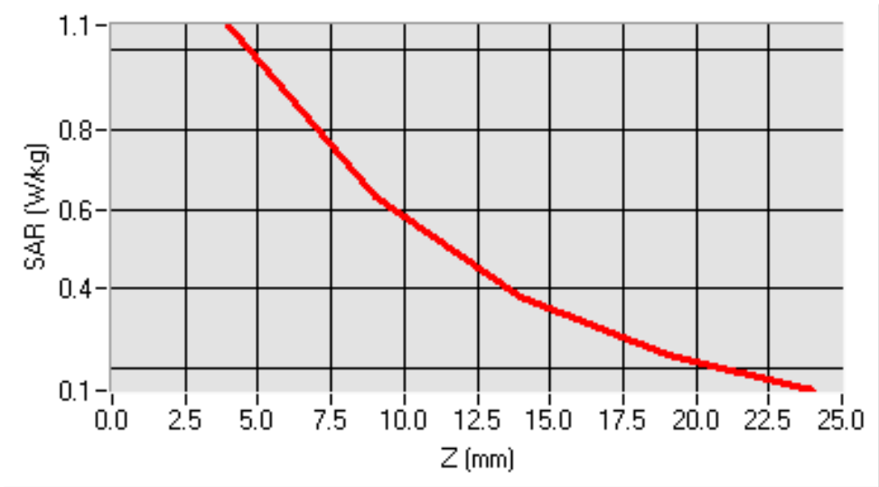
SAR, Z Axis Scan (X = -55, Y = -38)
