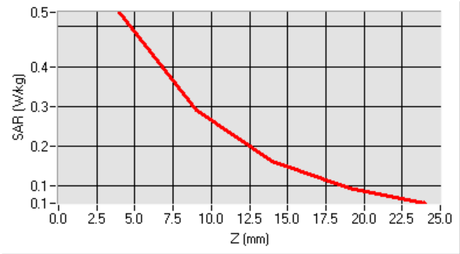
SAR, Z Axis Scan (X = 8, Y = -18)
