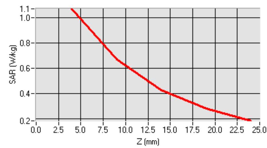
SAR, Z Axis Scan (X = -54, Y = -35)
