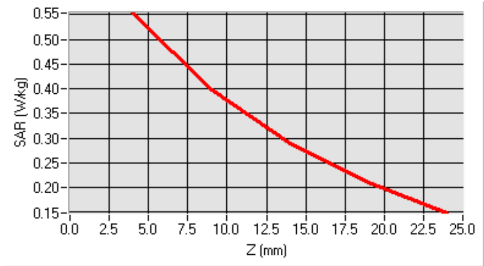
SAR, Z Axis Scan (X = 2, Y = -33)
