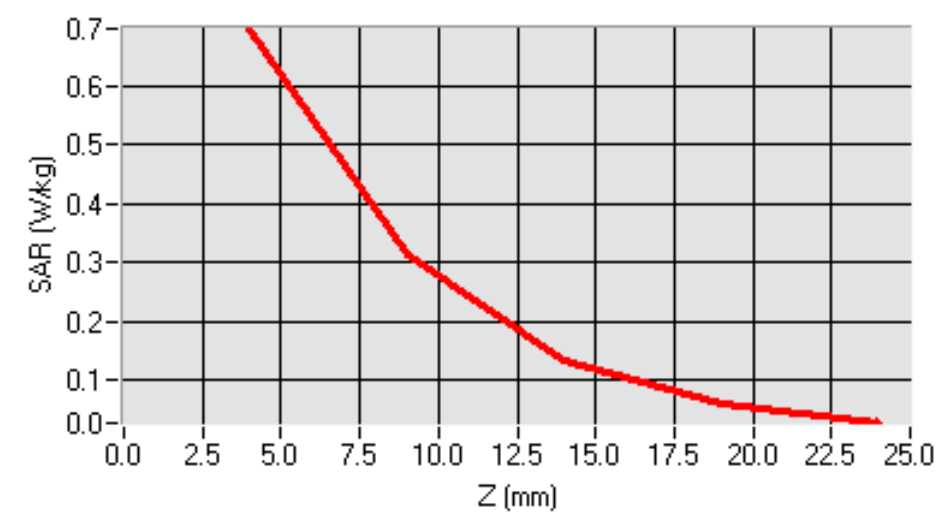
SAR, Z Axis Scan (X = -6, Y = -2)
