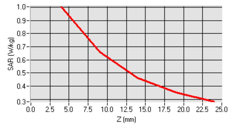
SAR, Z Axis Scan (X = -5, Y = -7)
