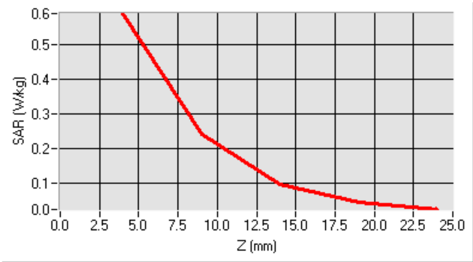
SAR, Z Axis Scan (X = -22, Y = 5)
