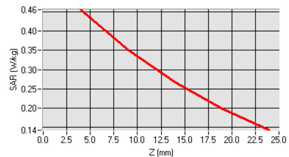
SAR, Z Axis Scan (X = 6, Y = -25)
