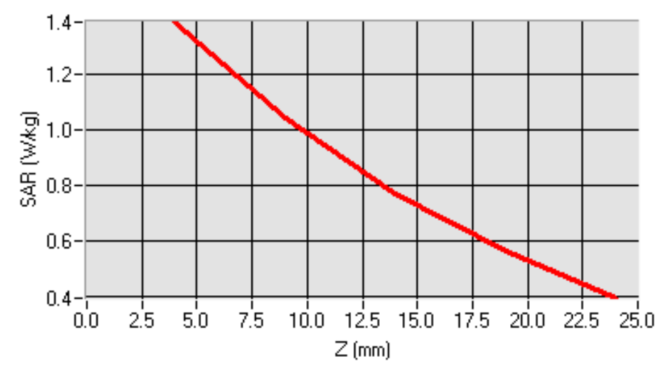
SAR, Z Axis Scan (X = -16, Y = -9)
