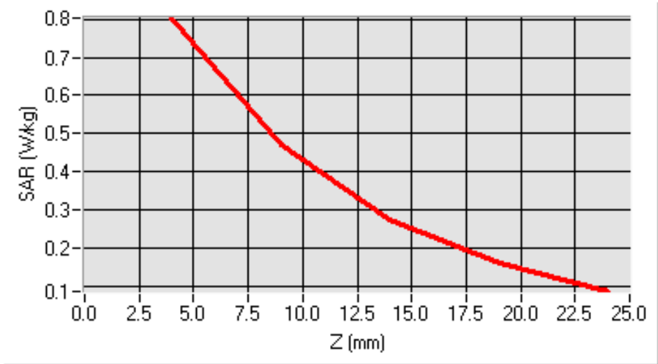
SAR, Z Axis Scan (X = -2, Y = 15)
