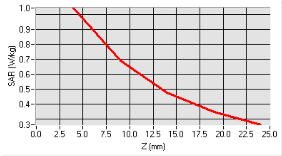
SAR, Z Axis Scan (X = 13, Y = -22)
