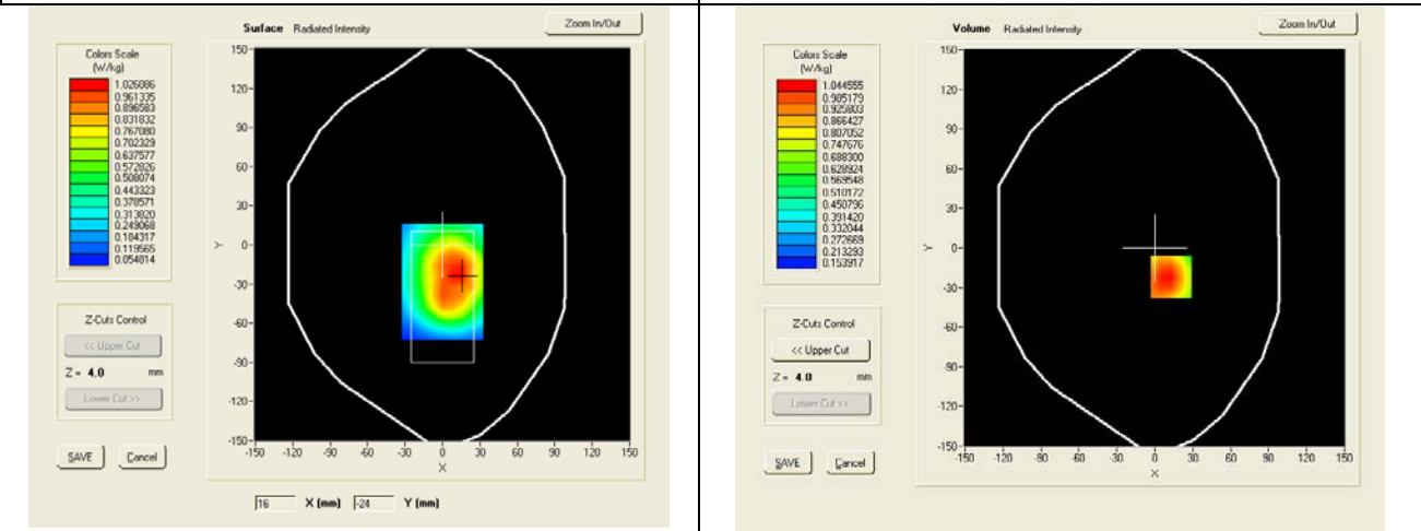
SAR, Z Axis Scan (X = 13, Y = -22)
