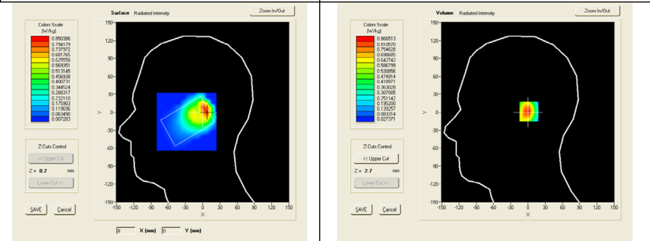
SAR, Z Axis Scan (X = 7, Y = 1)
