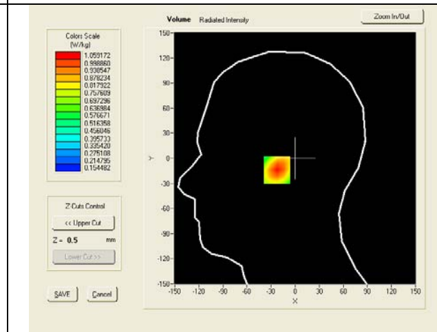
SAR, Z Axis Scan (X = -18, Y = -14)
