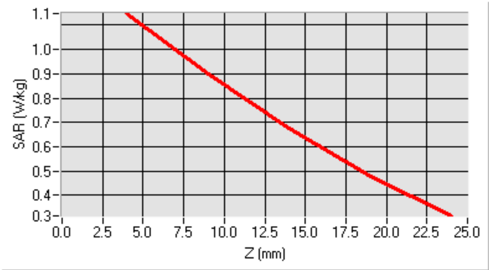
SAR, Z Axis Scan (X = -19, Y = -7)
