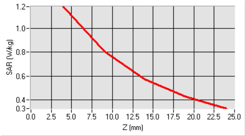
SAR, Z Axis Scan (X = 8, Y = -25)
