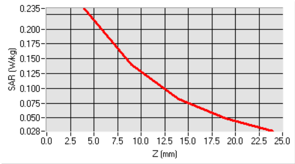
SAR, Z Axis Scan (X = -17, Y = -39)
