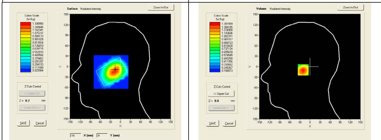
SAR, Z Axis Scan (X = -16, Y = -9)
