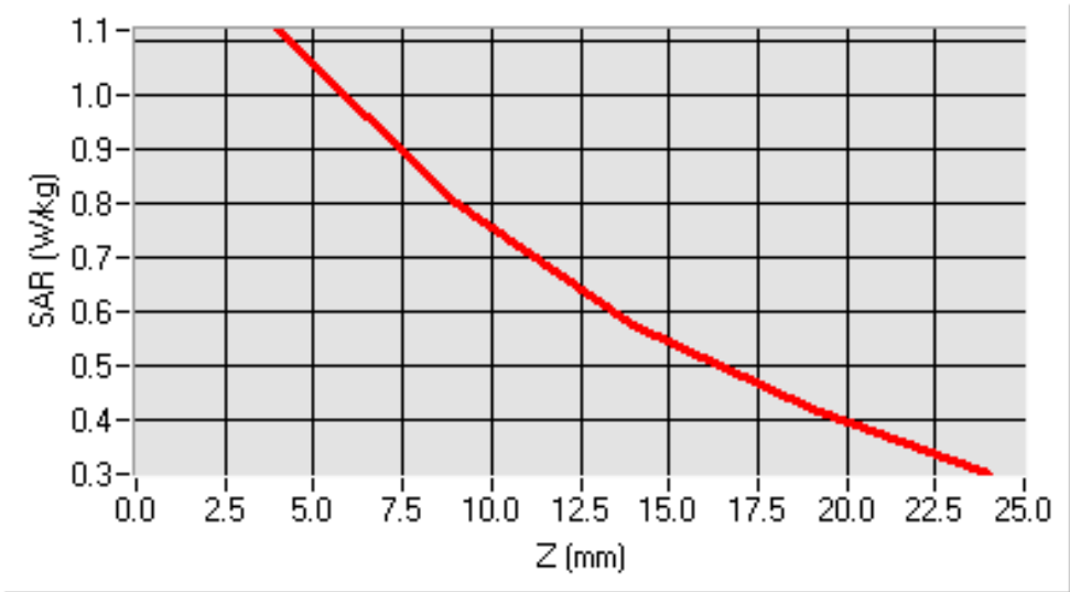
SAR, Z Axis Scan (X = 9, Y = -24)
