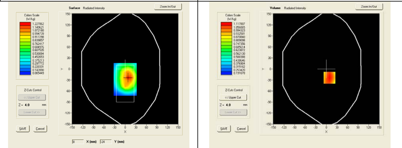
SAR, Z Axis Scan (X = 9, Y = -24)
