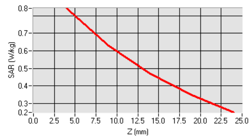
SAR, Z Axis Scan (X = -9, Y = -9)
