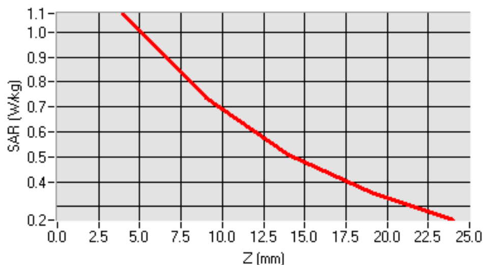
SAR, Z Axis Scan (X = -20, Y = 2)
