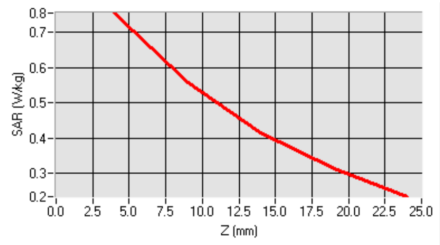
SAR, Z Axis Scan (X = -1, Y = -10)
