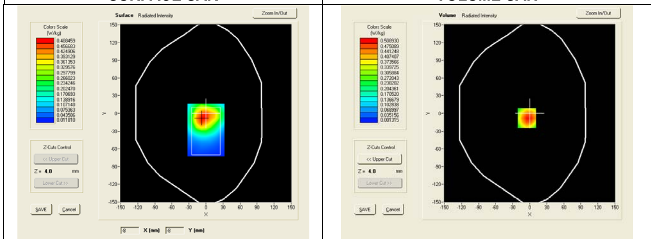
SAR, Z Axis Scan (X = -5, Y = -8)
