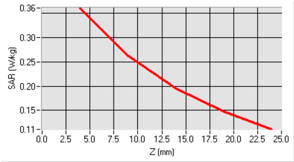
SAR, Z Axis Scan (X = -22, Y = -3)
