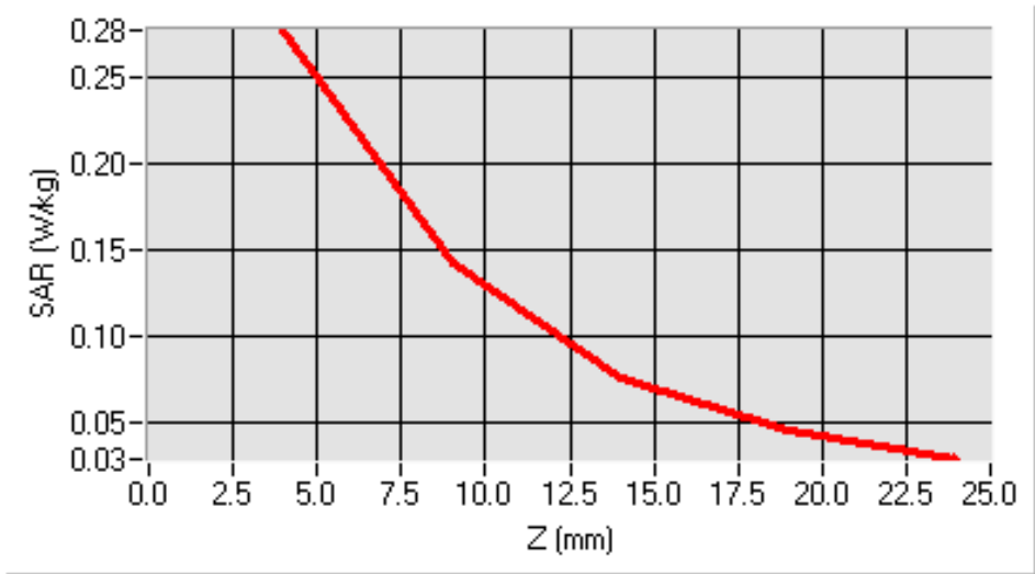
SAR, Z Axis Scan (X = -8, Y = 3)
