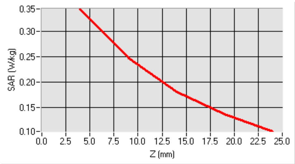
SAR, Z Axis Scan (X = 0, Y = -31)
