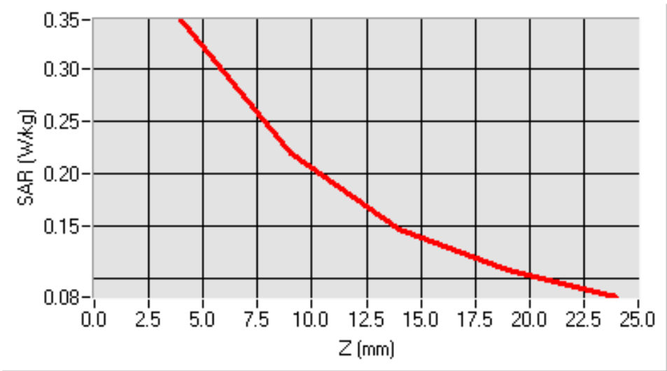
SAR, Z Axis Scan (X = -6, Y = -8)
