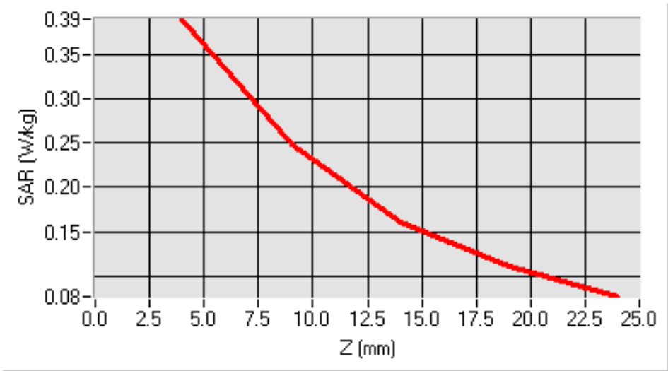
SAR, Z Axis Scan (X = -18, Y = 14)
