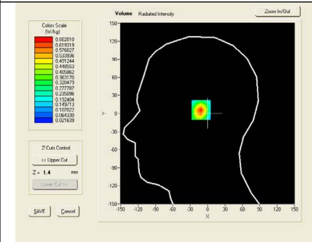
SAR, Z Axis Scan (X = -8, Y = 6)
