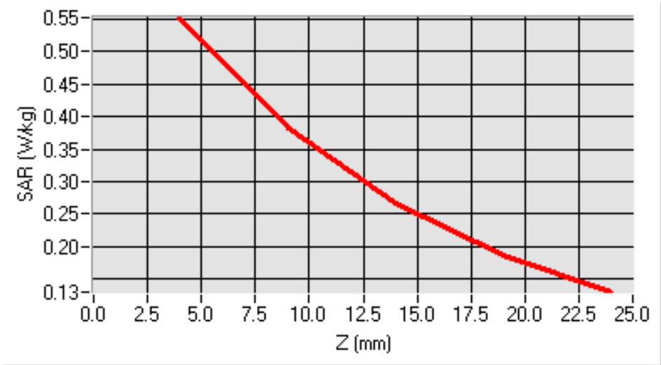
SAR, Z Axis Scan (X = -20, Y = -10)
