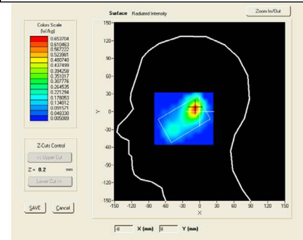
SAR, Z Axis Scan (X = -8, Y = 6)
