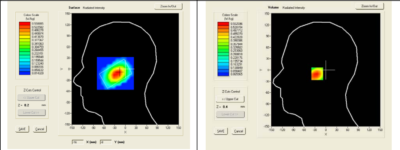
SAR, Z Axis Scan (X = -20, Y = -10)
