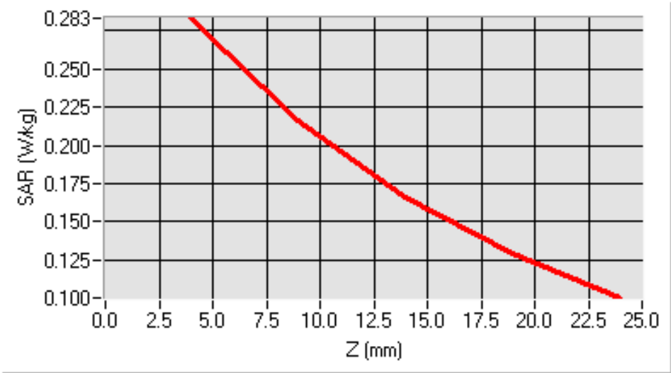
SAR, Z Axis Scan (X = 6, Y = -41)
