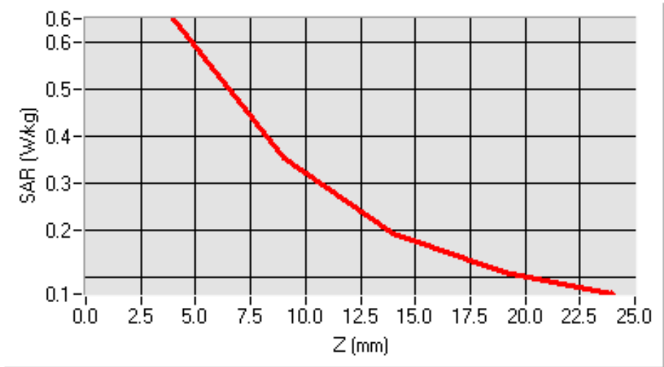
SAR, Z Axis Scan (X = -6, Y = 7)
