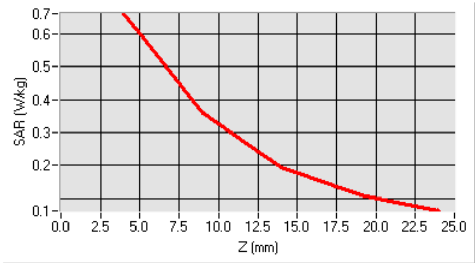
SAR, Z Axis Scan (X = -8, Y = 6)
