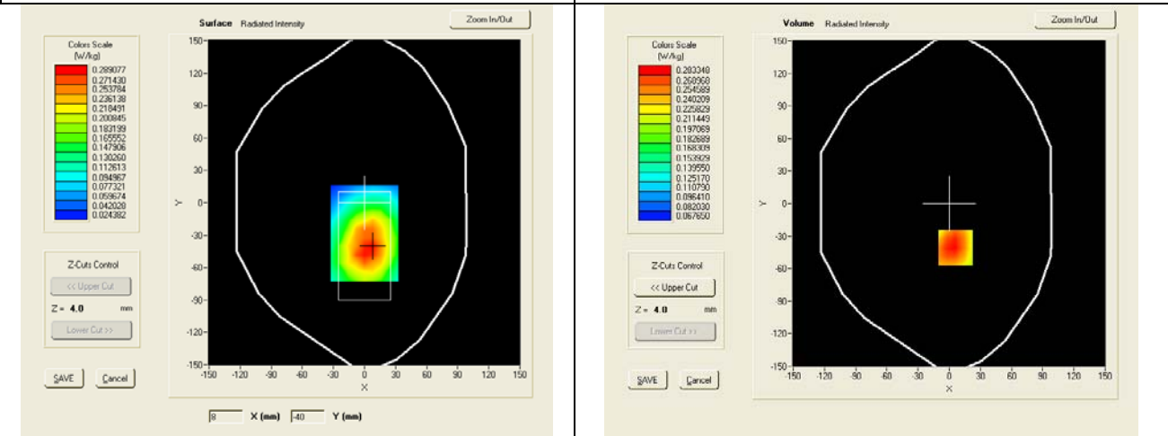
SAR, Z Axis Scan (X = 6, Y = -41)
