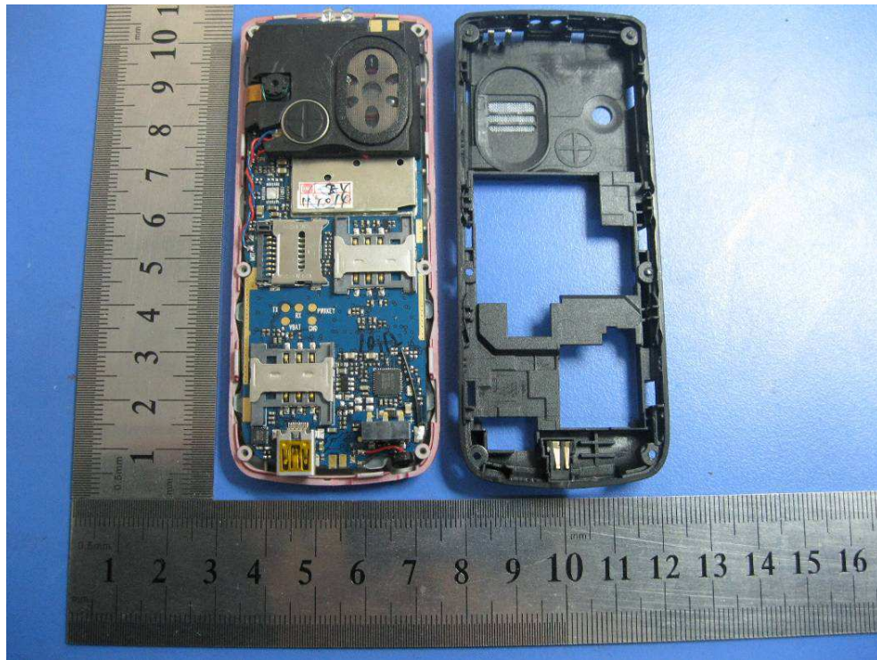
EUT –Rear Cover Off View
