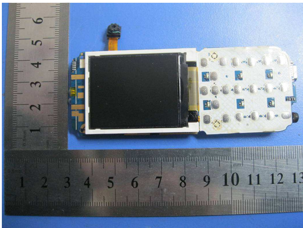
EUT – Main Board With LCD Bottom View
